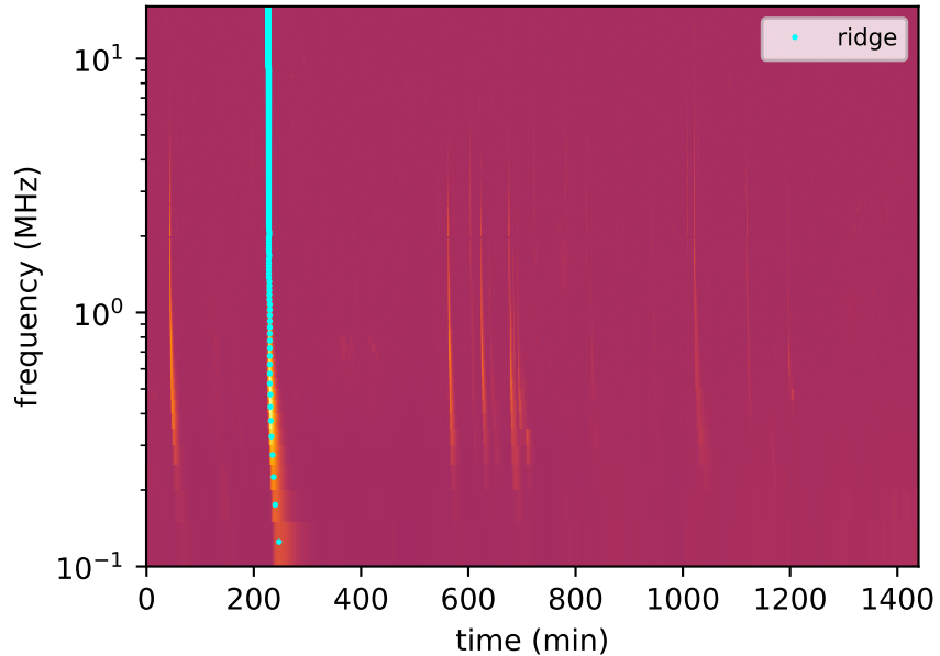
STEREO/WAVES type III
