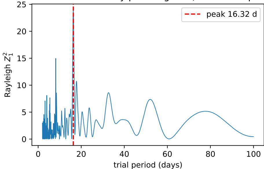
FRB20180916B activity periodogram (14 transit epochs)
