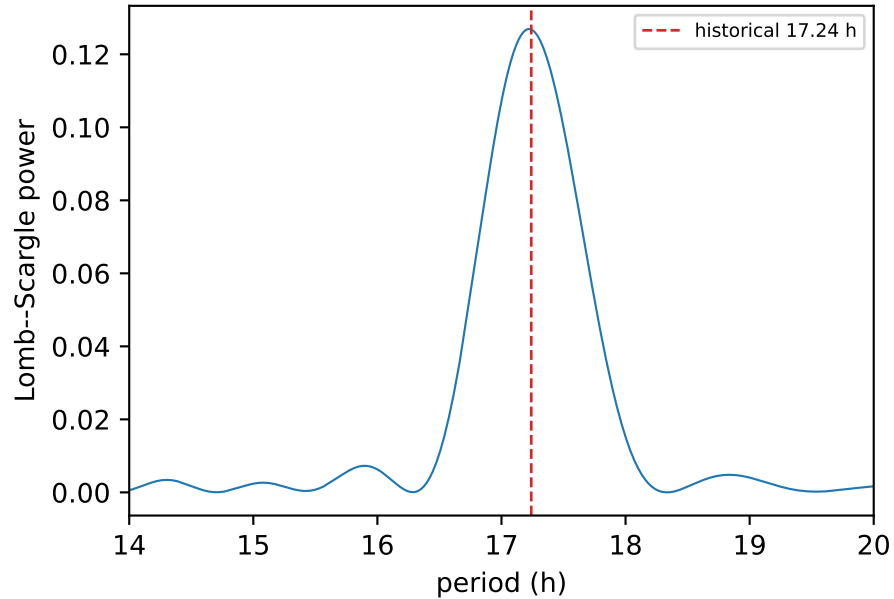
Synthetic control
