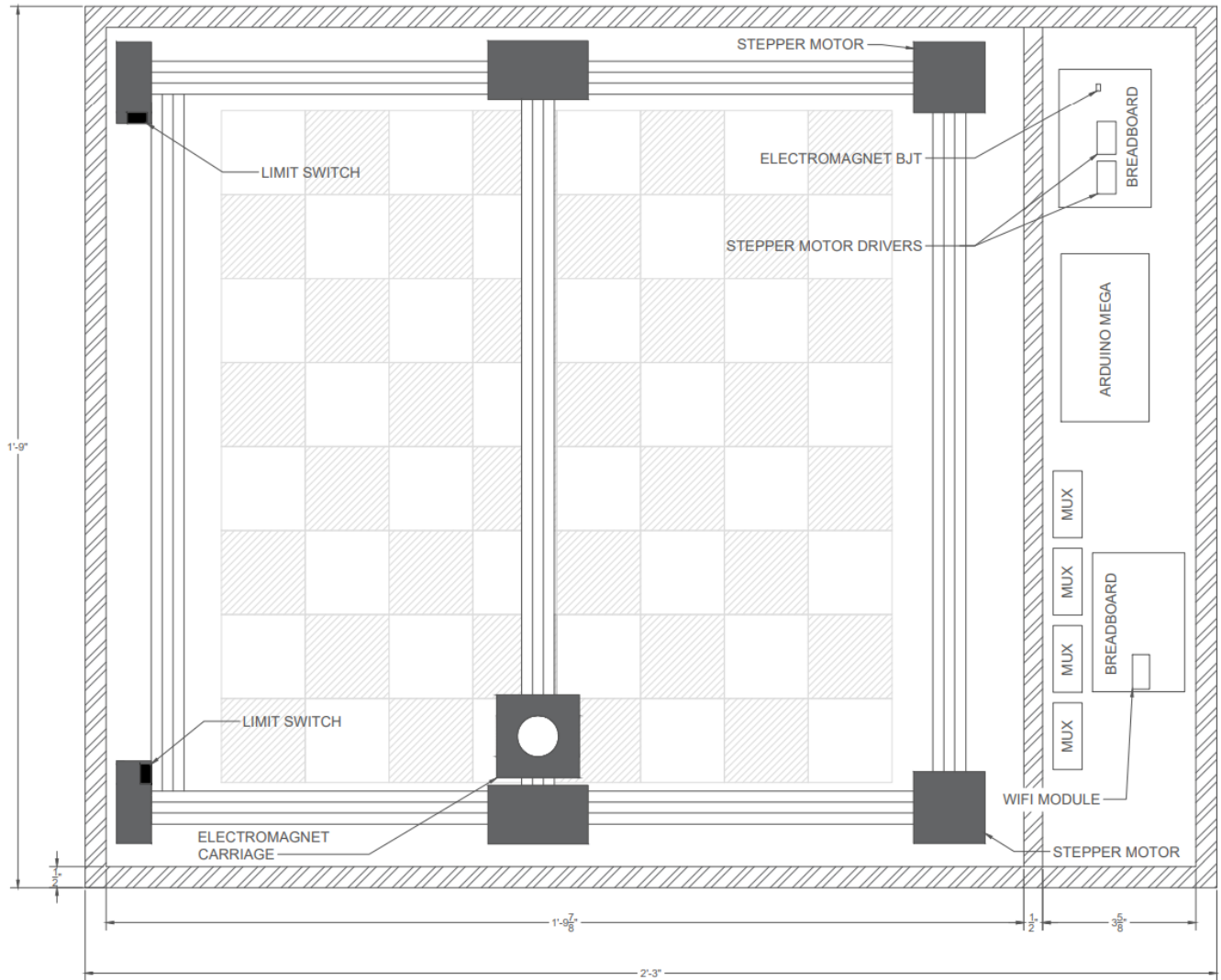
Fig. 2: Internal view of ChessConnect
