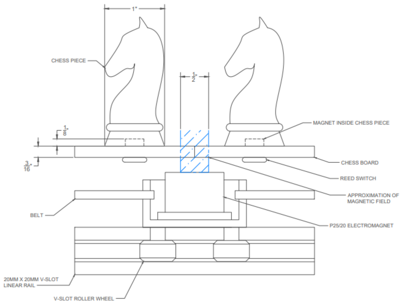
Fig. 3: Enlarged side view of ChessConnect
