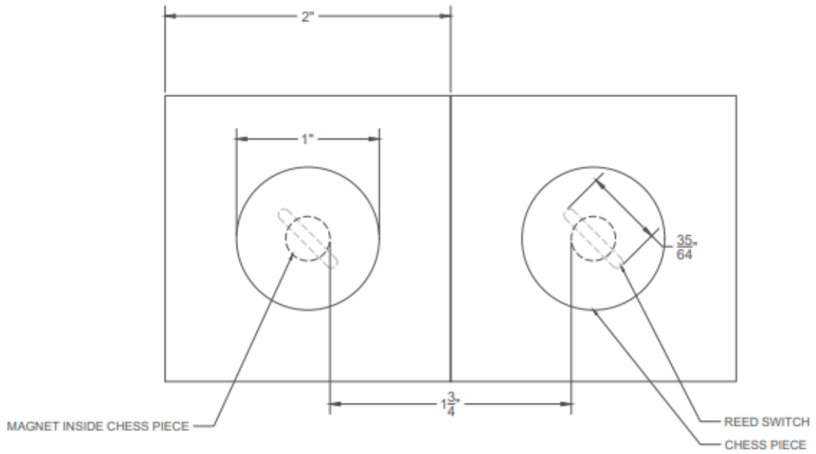
Fig. 4: Enlarged top view of ChessConnect
