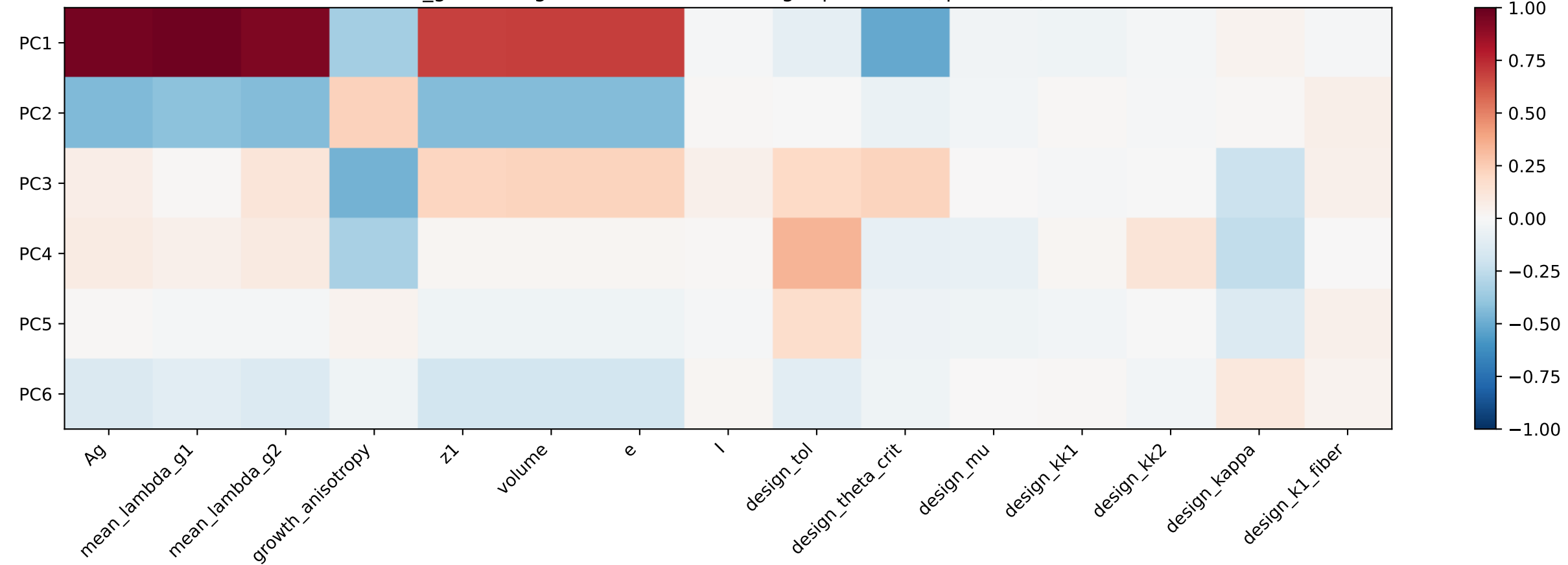
h_g PCs vs. growth/mechanical/design quantities (Spearman)
