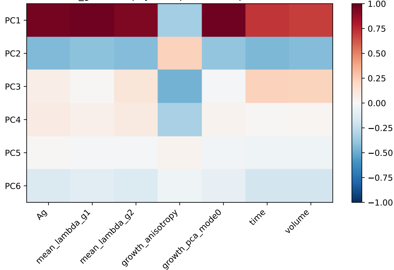
h_g PCs vs. physical quantities (Spearman)
