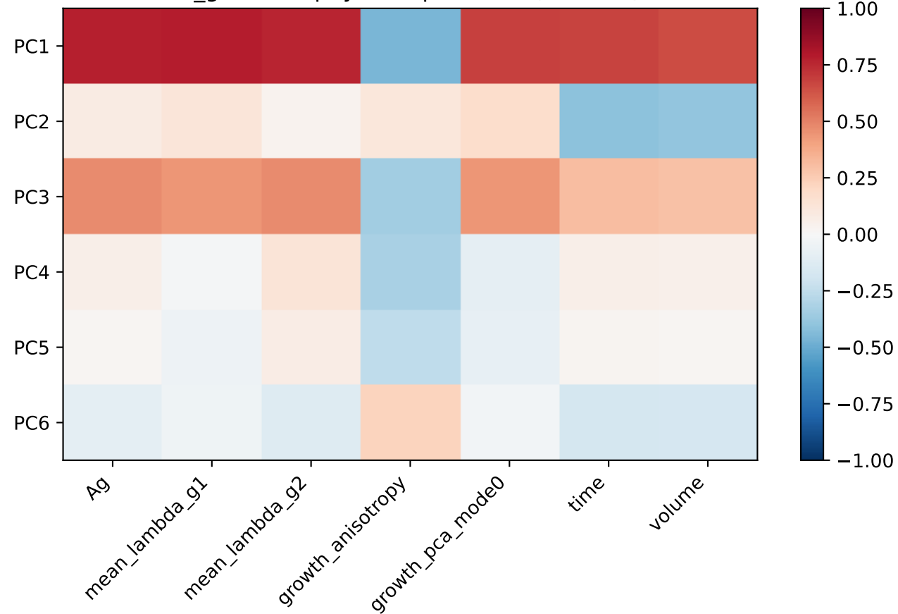
h_g PCs vs. physical quantities (Pearson)
