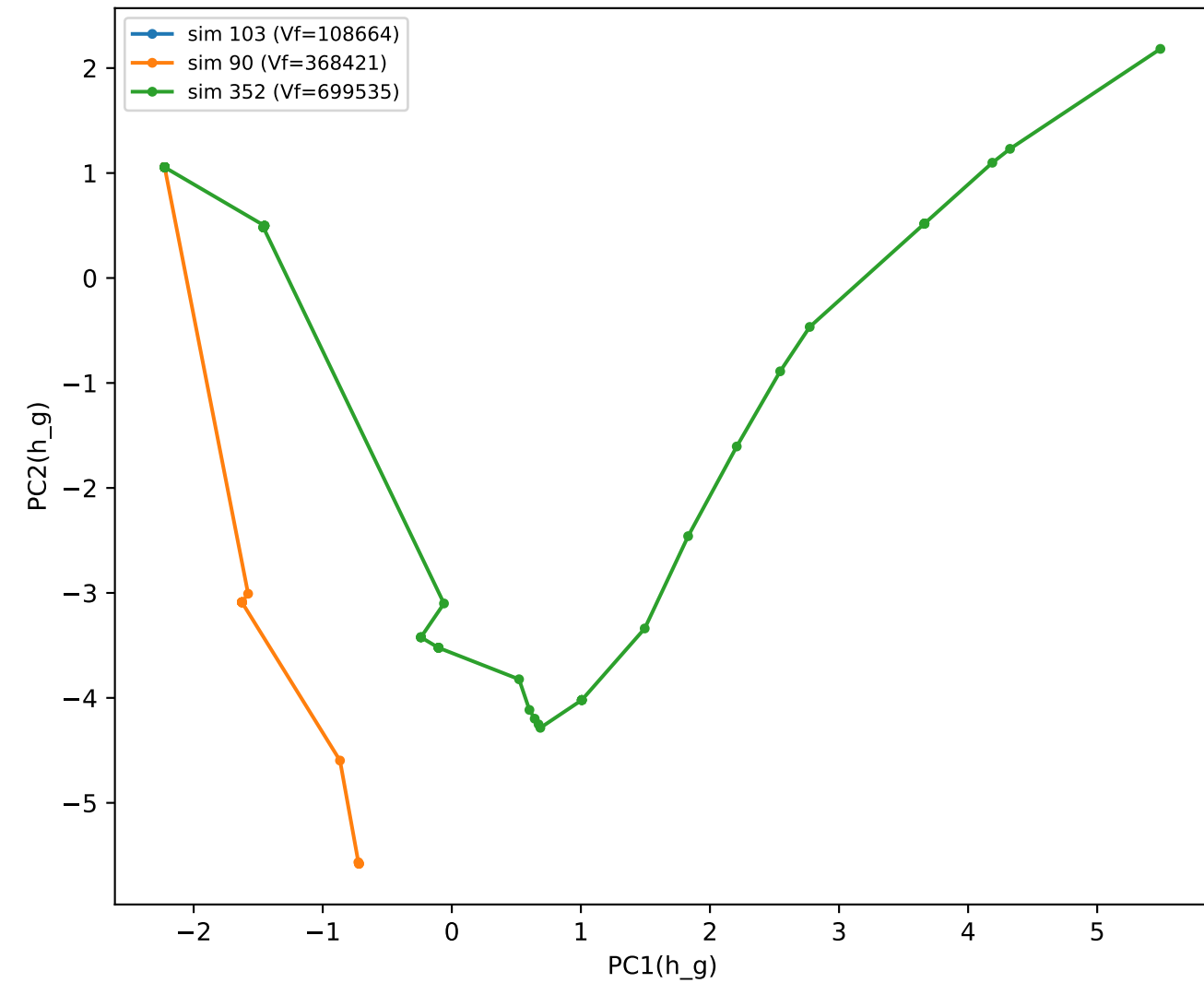
CNN-feature trajectories
