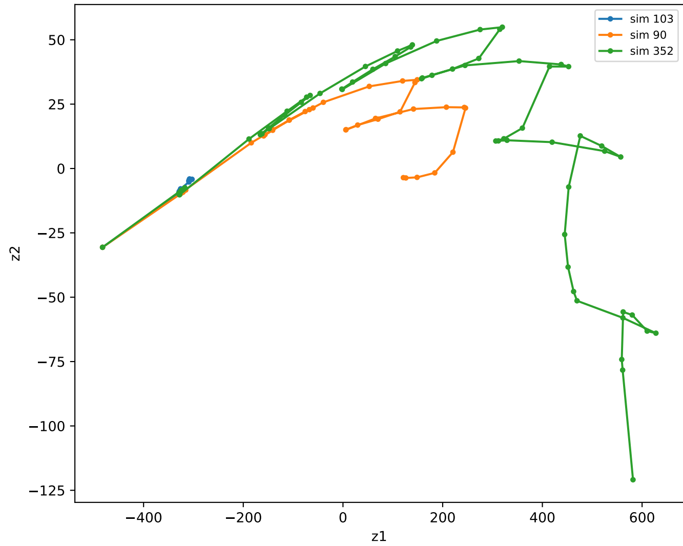
Mechanical-latent trajectories
