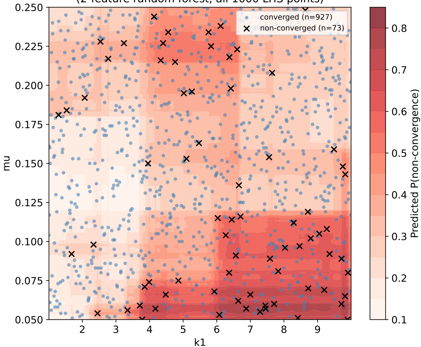
FE non-convergence probability: k1 vs mu (2-feature random forest, all 1000 LHS points)
