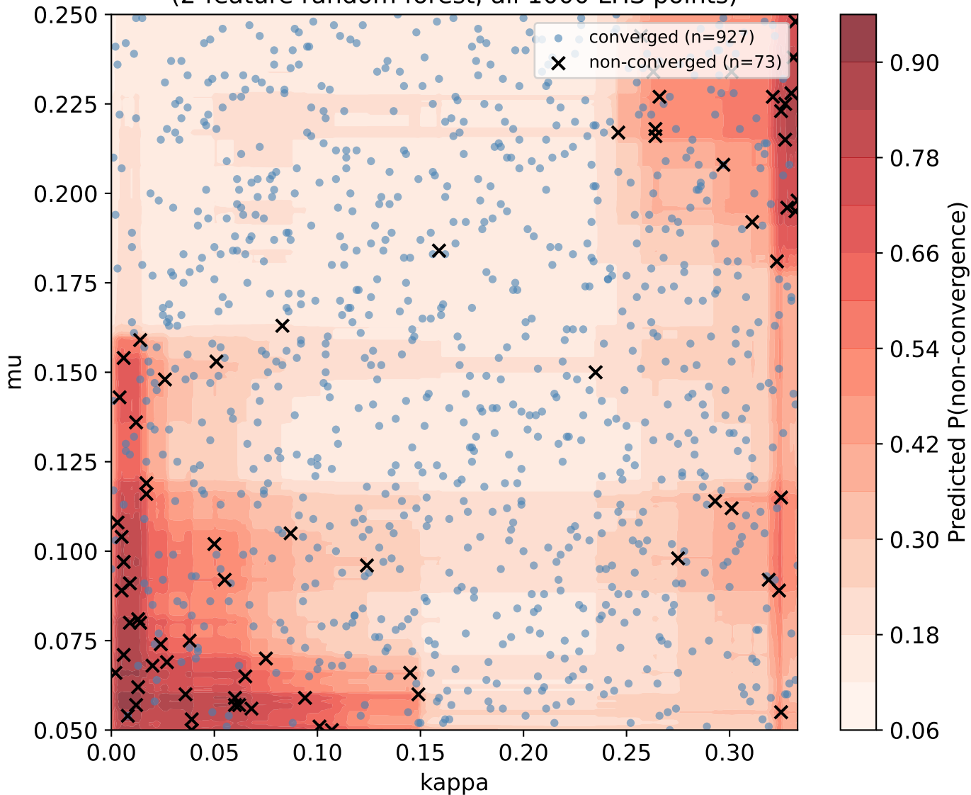
FE non-convergence probability: kappa vs mu (2-feature random forest, all 1000 LHS points)
