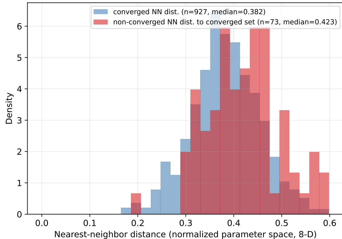
Nearest-neighbor distance distributions
