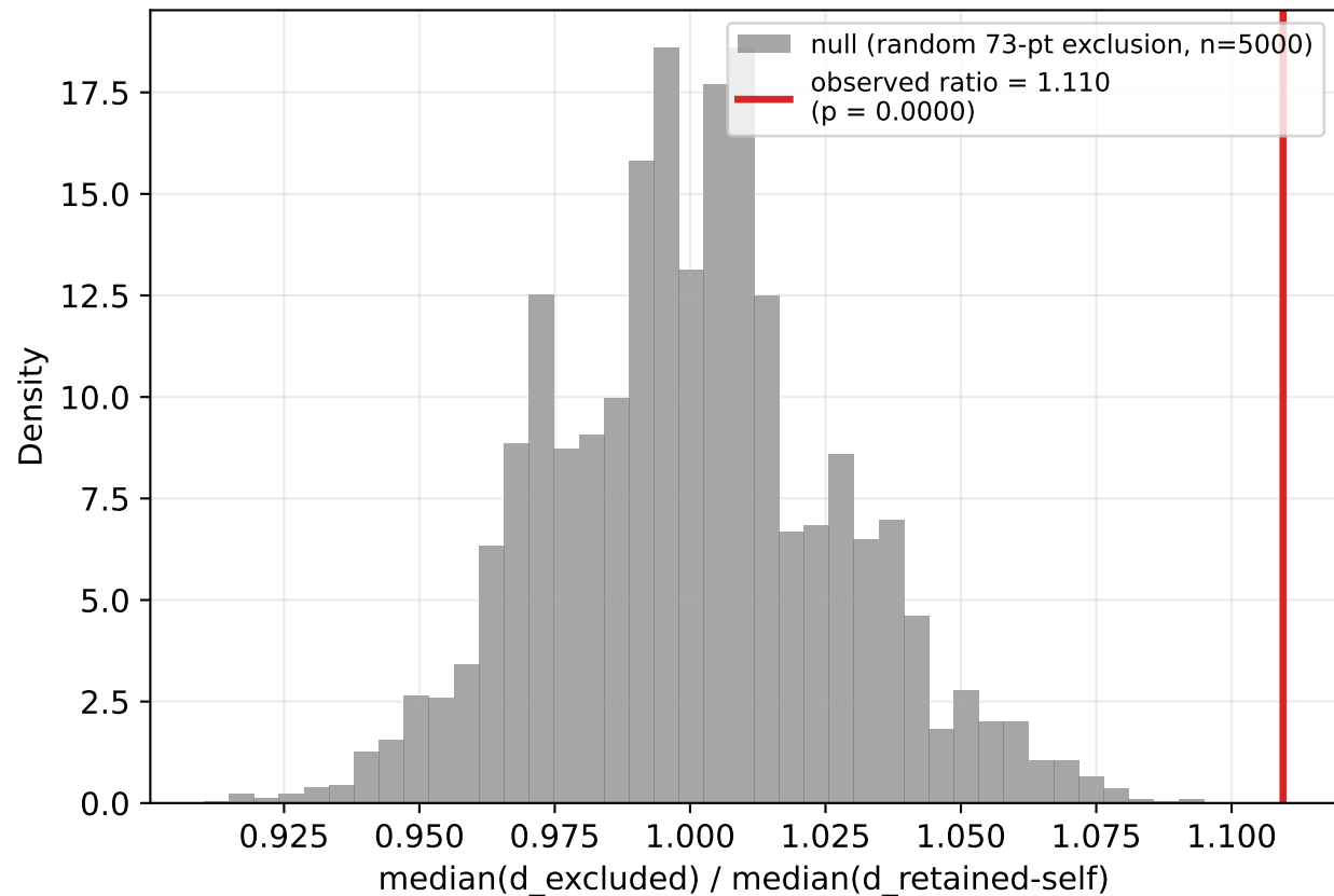
Permutation test: is the observed ratio more extreme than random exclusion?
