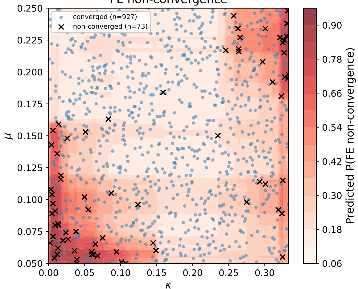
FE non-convergence
