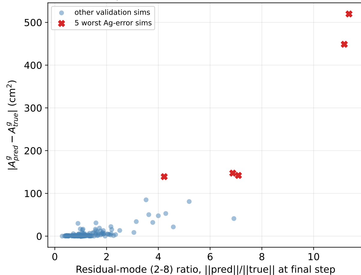
Residual growth-PCA-mode blow-up vs. Ag error (Spearman rho=0.52, Pearson r=0.87)
