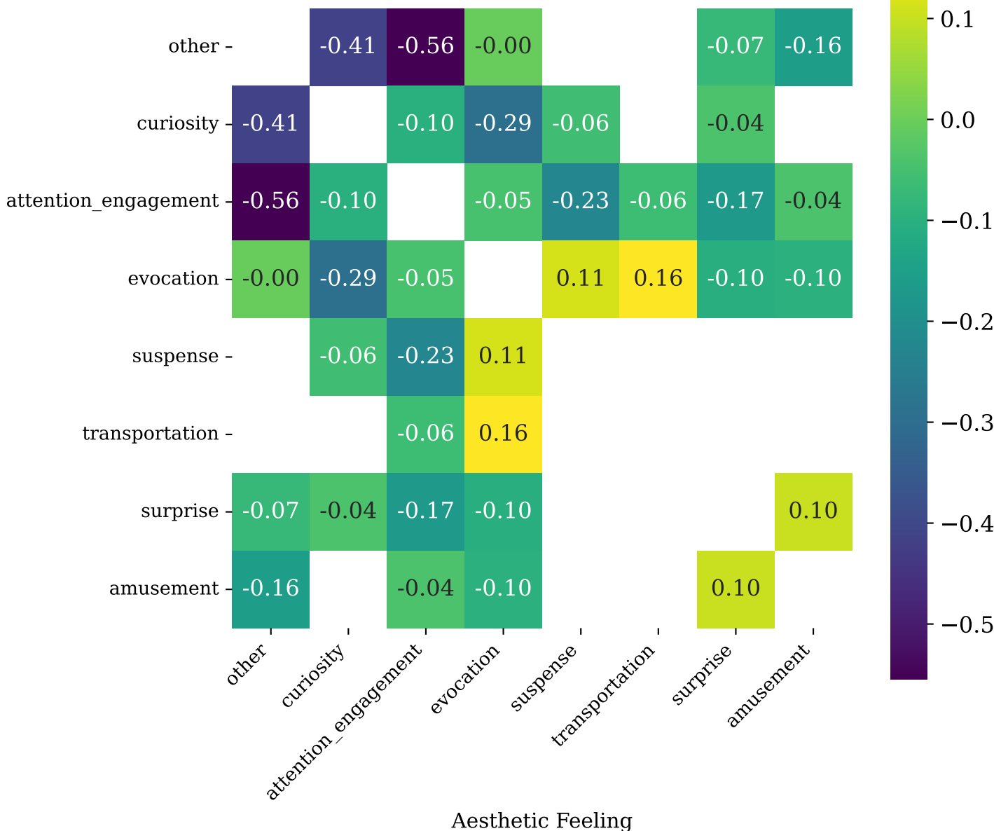
Inter-dimension Associations: aesthetic_feeling × aesthetic_feeling (clustered)
