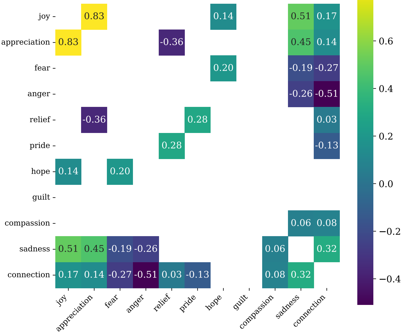
Inter-dimension Associations: author_emotional_response × author_emotional_response (clustered)
