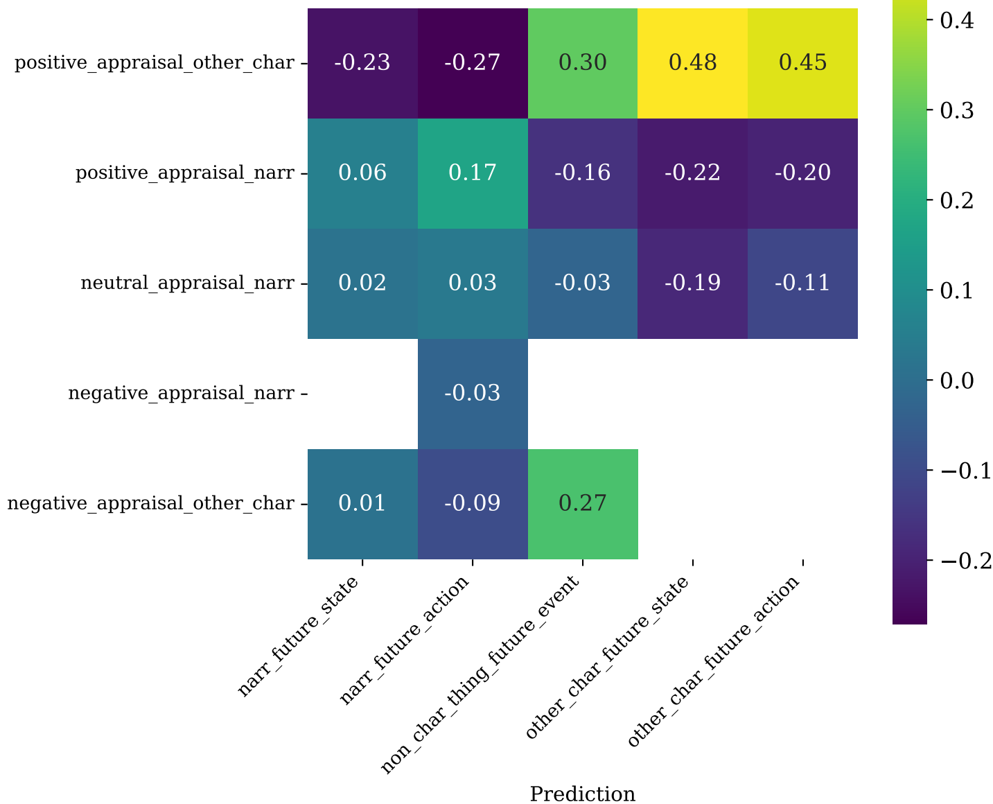
Inter-dimension Associations: character_appraisal × prediction (clustered)
