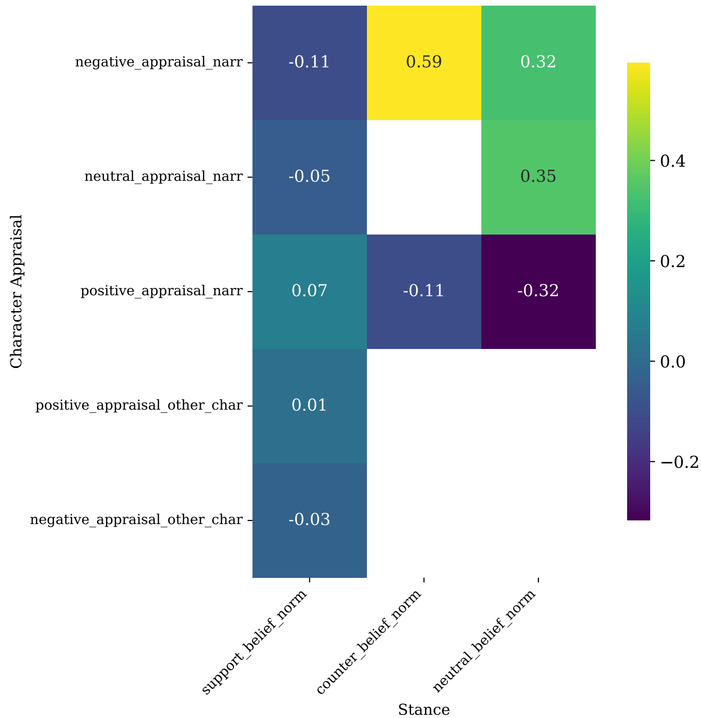
Inter-dimension Associations: character_appraisal × stance (clustered)
