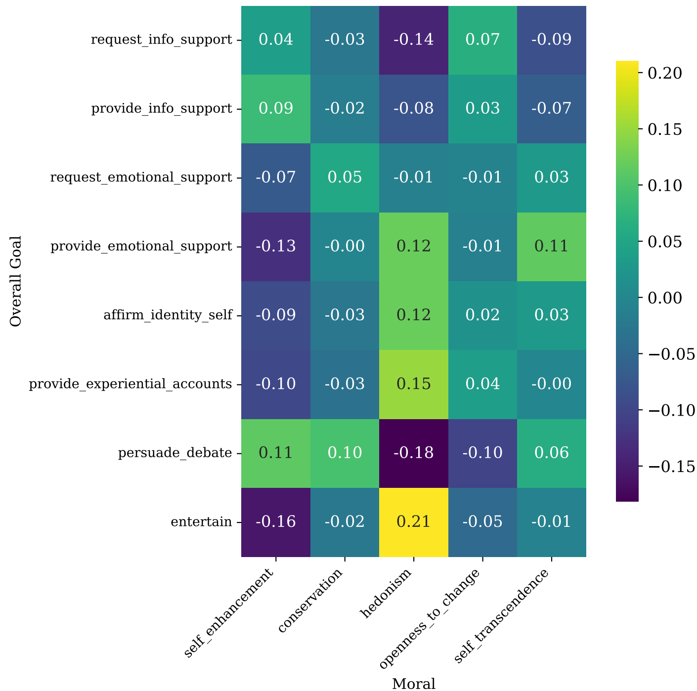
Inter-dimension Associations: overall_goal × moral
