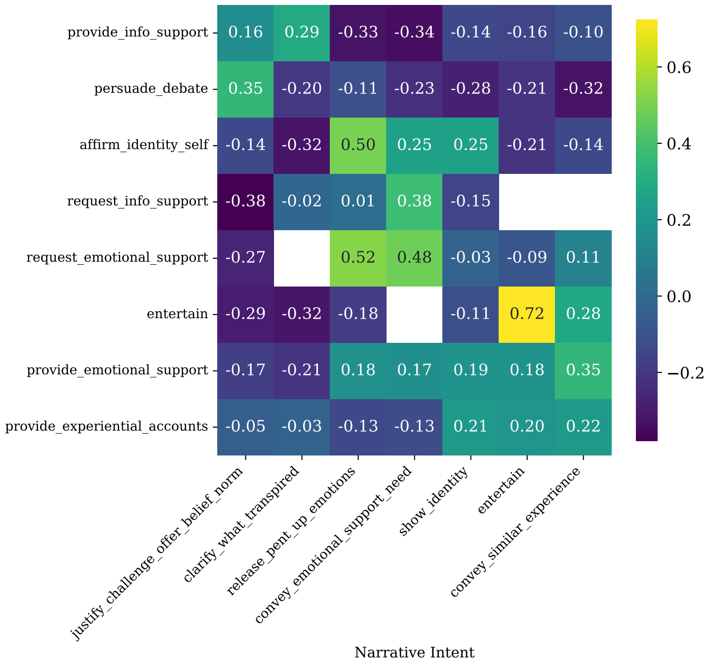
Inter-dimension Associations: overall_goal × narrative_intent (clustered)
