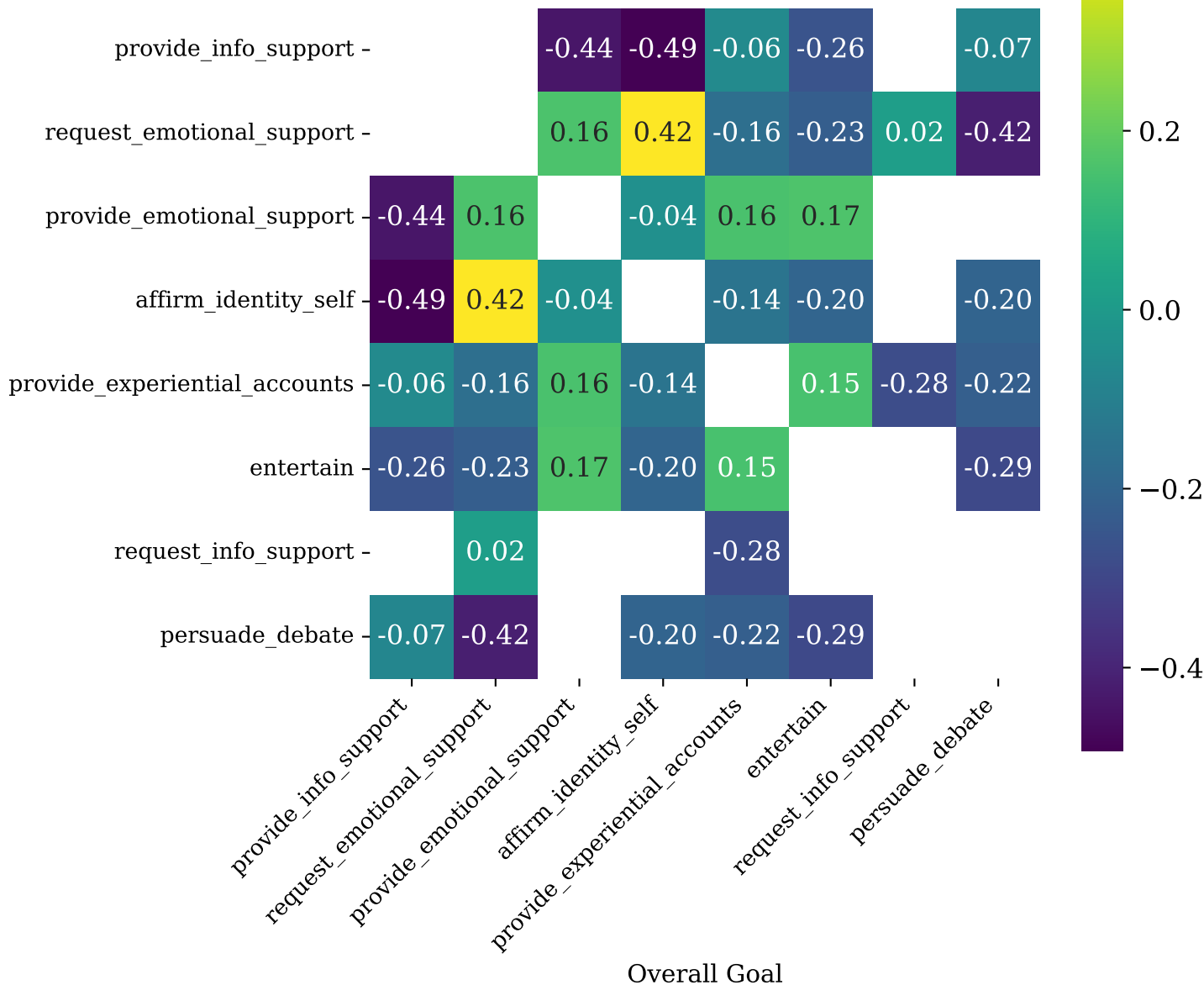
Inter-dimension Associations: overall_goal × overall_goal (clustered)
