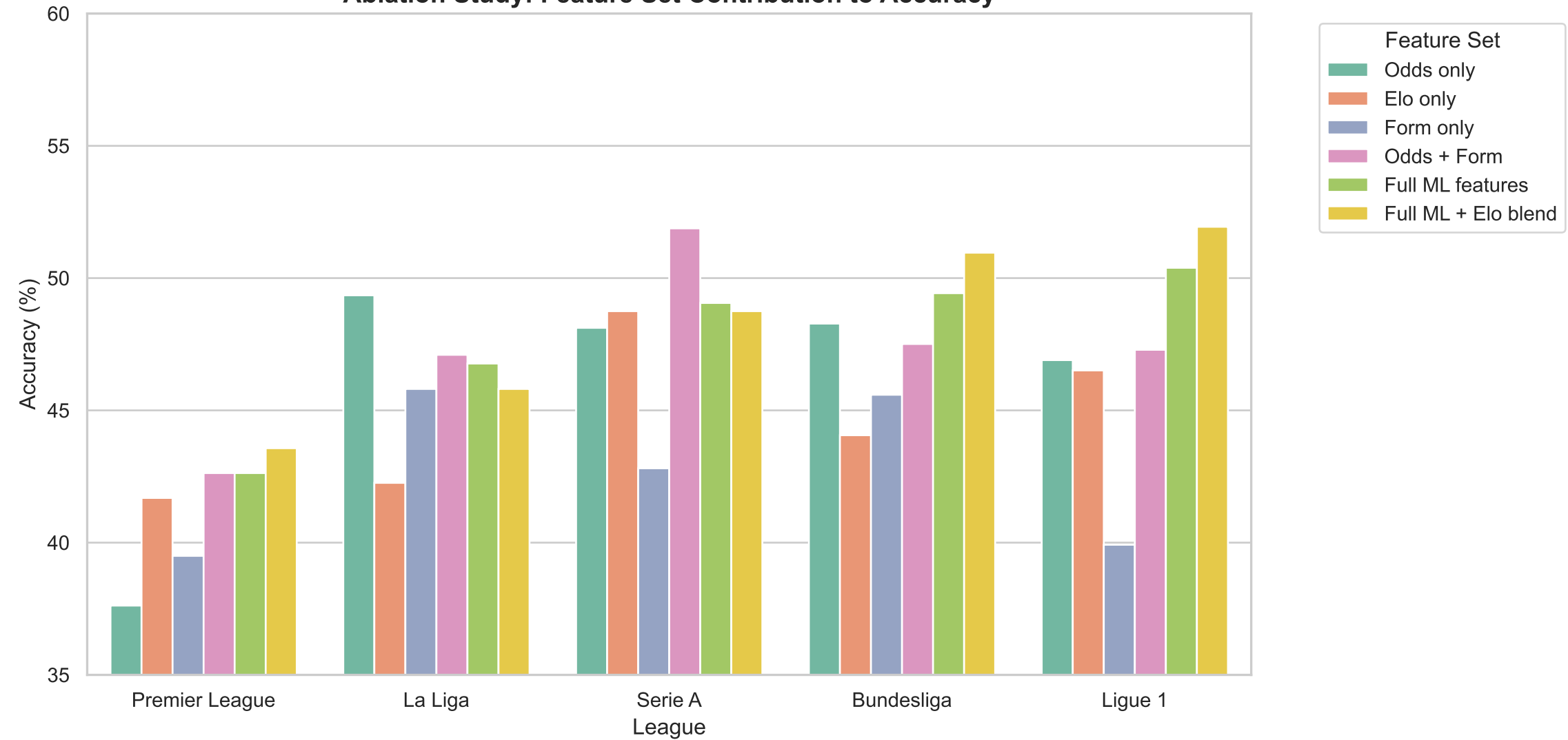
Ablation Study: Feature Set Contribution to Accuracy
