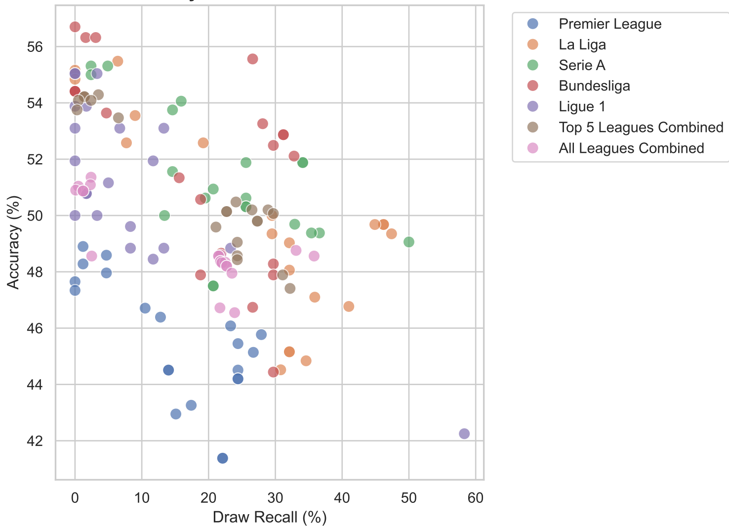
Accuracy vs. Draw Recall Trade-off
