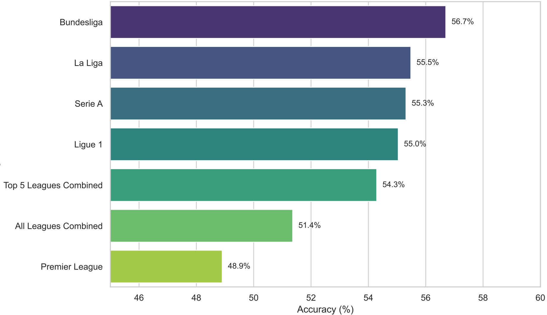
Best Model Accuracy per Scenario (2025/26 Holdout)
