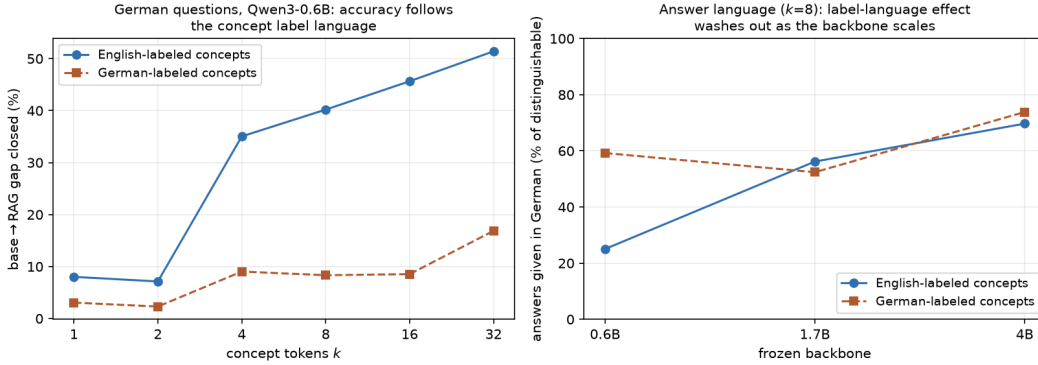
Figure 8: German PopQA (14,230 questions, German system prompt, German entity mention). Left: on Qwen3-0.6B, base \rightarrow RAG gap closure across k for concepts built from English vs. German entity labels. Right: at k=8 , the share of correct answers given in German (of those where the German and English answer forms differ), by backbone.
