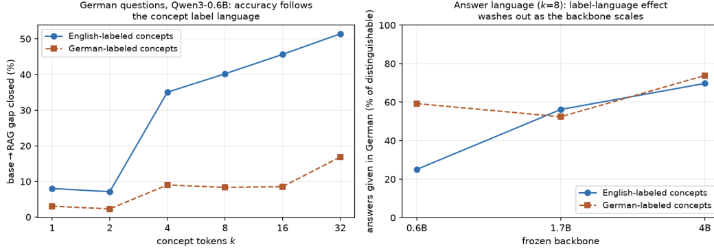
Figure 8: German PopQA (14,230 questions, German system prompt, German entity mention). Left: on Qwen3-0.6B, base→RAG gap closure across k for concepts built from English vs. German entity labels. Right: at k=8 , the share of correct answers given in German (of those where the German and English answer forms differ), by backbone.
