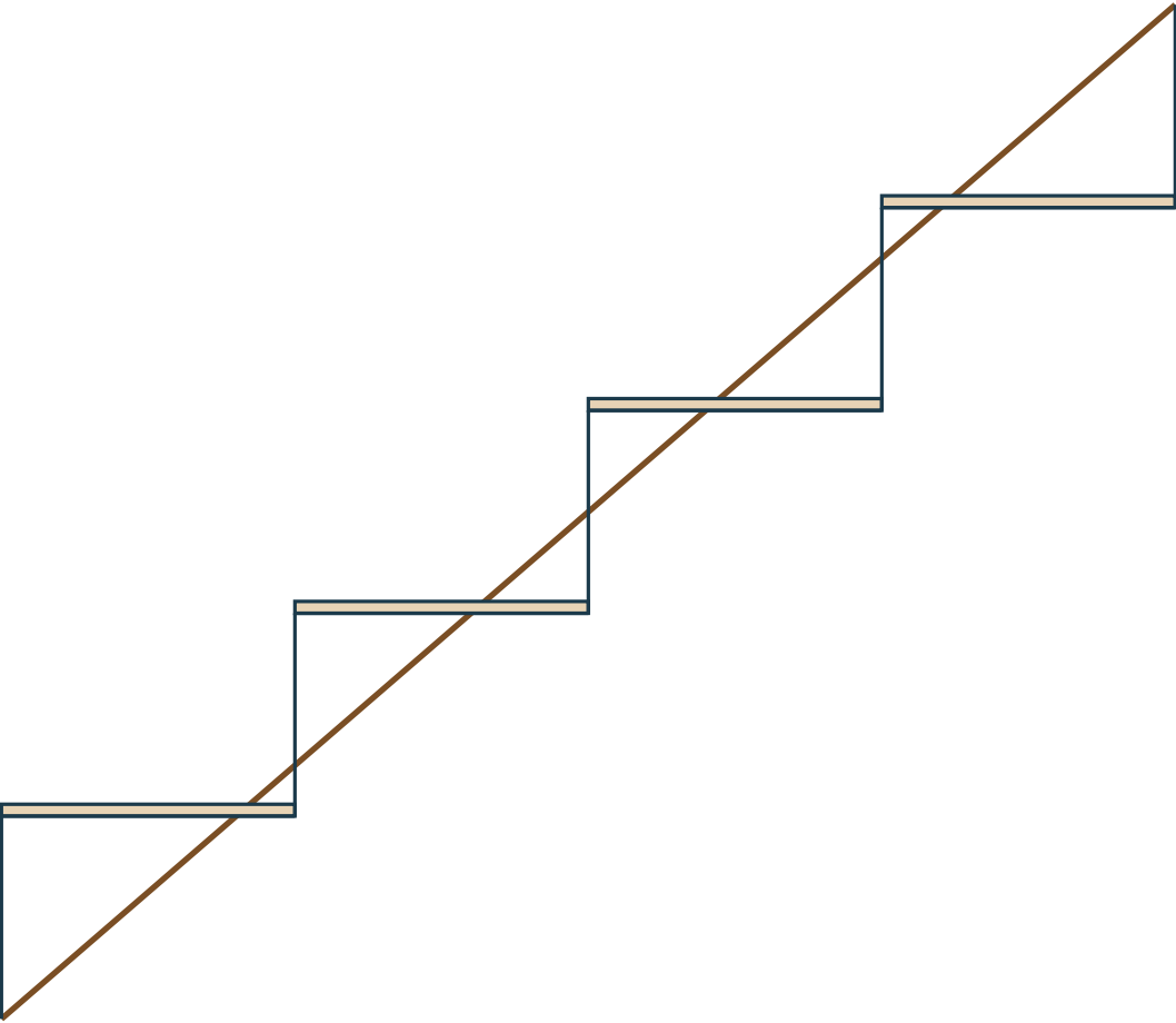
Total run 3'-8" Total rise 3'-2" Stringer cut basis 58.1 in Each tread is two 5/4 × 6 boards, 10 ft long. No centre handrail.
