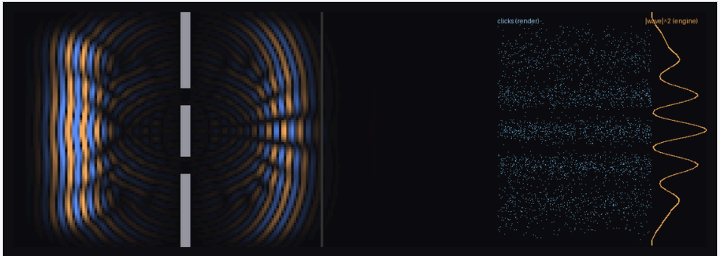
Figure 13. Duality as architecture. Left: the engine's wave interferes through both slits. Right: the renderer's discrete clicks reproduce |\text{wave}|^2 statistically.
