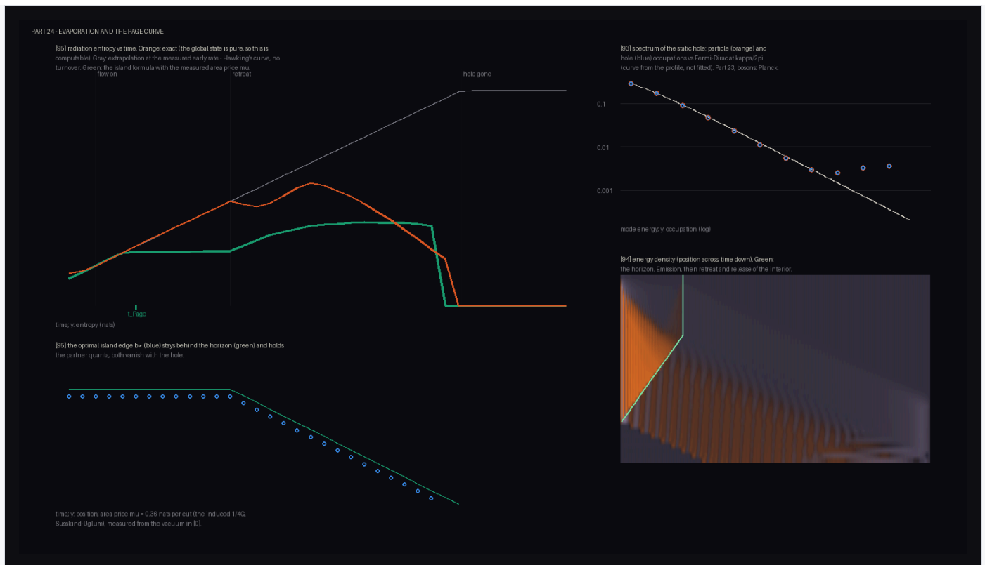
Figure 12. Evaporation. Left: the three entropy curves — exact (orange: rise, turnover, return to zero), the never-turning extrapolation (gray), and the island formula with the measured area term (green) — with the optimal island edge tracking the horizon below. Right: the Fermi–Dirac spectrum of the deep static hole, and the energy density over time showing emission, retreat, and the release of the interior.
