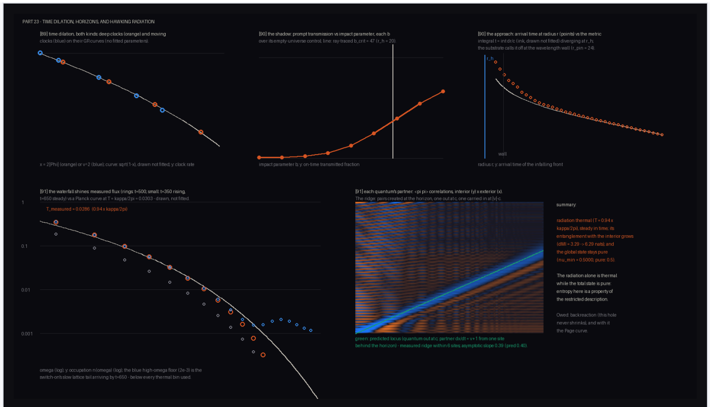
Figure 11. Horizons, measured. Top: both time dilations on their GR curves (no fitted parameters); the photon shadow against the ray-traced critical impact parameter; infalling light following the diverging metric integral until the lattice-scale cutoff. Bottom: the steady Hawking spectrum against a Planck curve at \kappa/2\pi (computed, not fitted), and the partner correlations — each emitted quantum's twin falling inside along the predicted trajectory.
