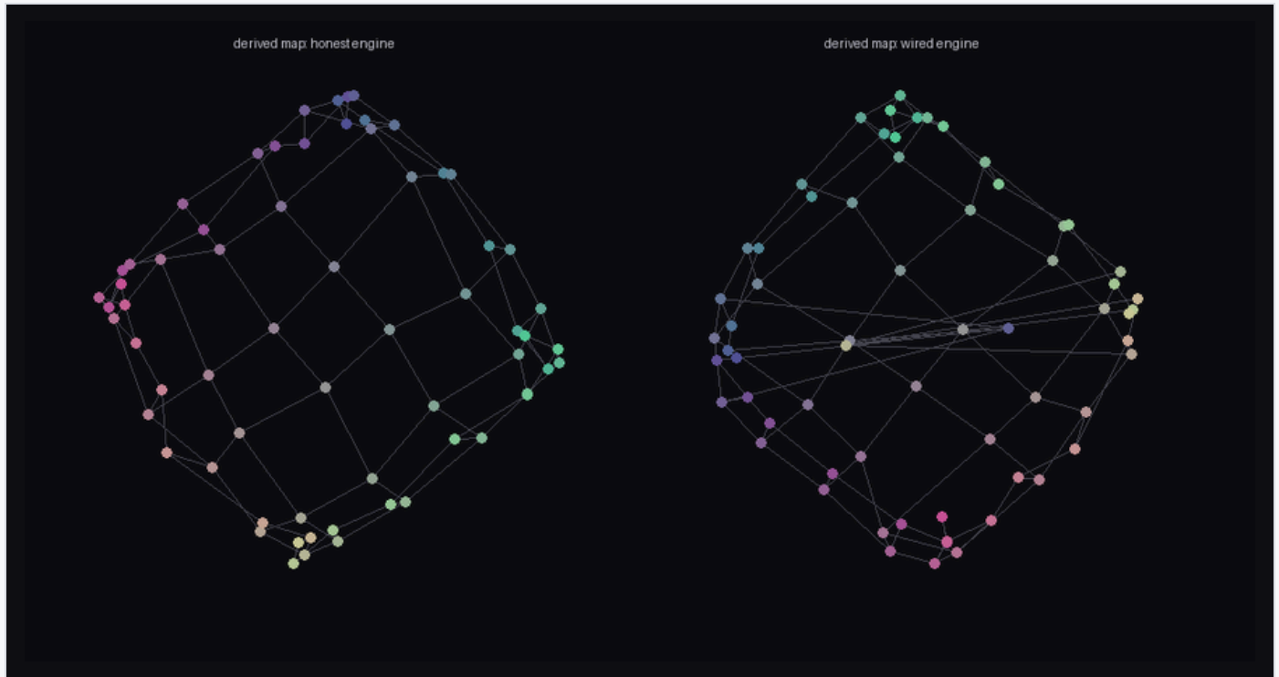
Figure 2. Geometry derived purely from causal structure (no cell index used as a position). Left: honest engine → flat mesh. Right: engine with a wired shortcut → the derived metric grows a wormhole.
