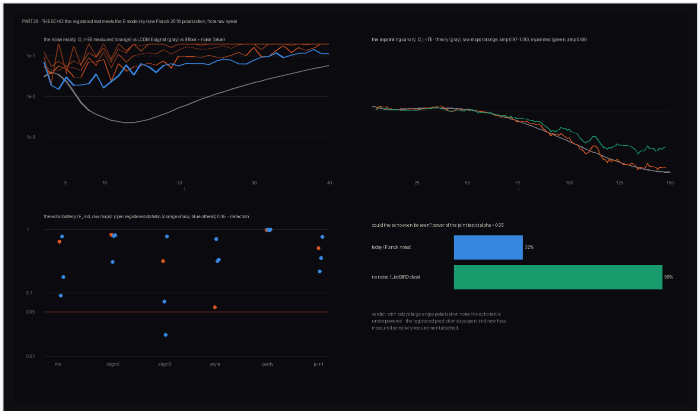
Figure 20. The echo test. Top left: the noise reality — measured EE (orange) sits on the B-mode floor (blue) rather than the \Lambda CDM E signal (gray) beyond \ell \approx 8 . Top right: the inpainting canary in TE. Bottom: the registered-axis battery (no echo) and the measured power of the test — 32% at today's noise, 98% at LiteBIRD-class.
