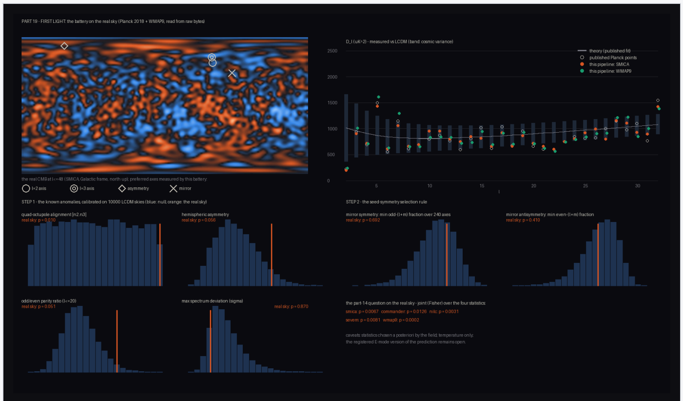
Figure 19. First light: the battery on the real sky. Left: the measured CMB (SMICA, \ell \leq 48 ) with the battery's preferred axes — the two rings nearly touching are the aligned quadrupole and octupole. Right: the from-raw-bytes spectrum against \Lambda CDM (the low quadrupole at far left). Below: each statistic against its 10,000-sky null (orange: the real sky).
