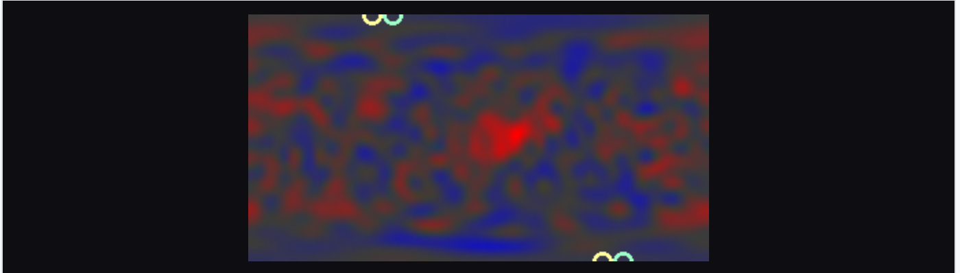
Figure 18. A synthetic sky carrying the three observed anomalies at published amplitudes; rings mark the aligned quadrupole and octupole axes.
