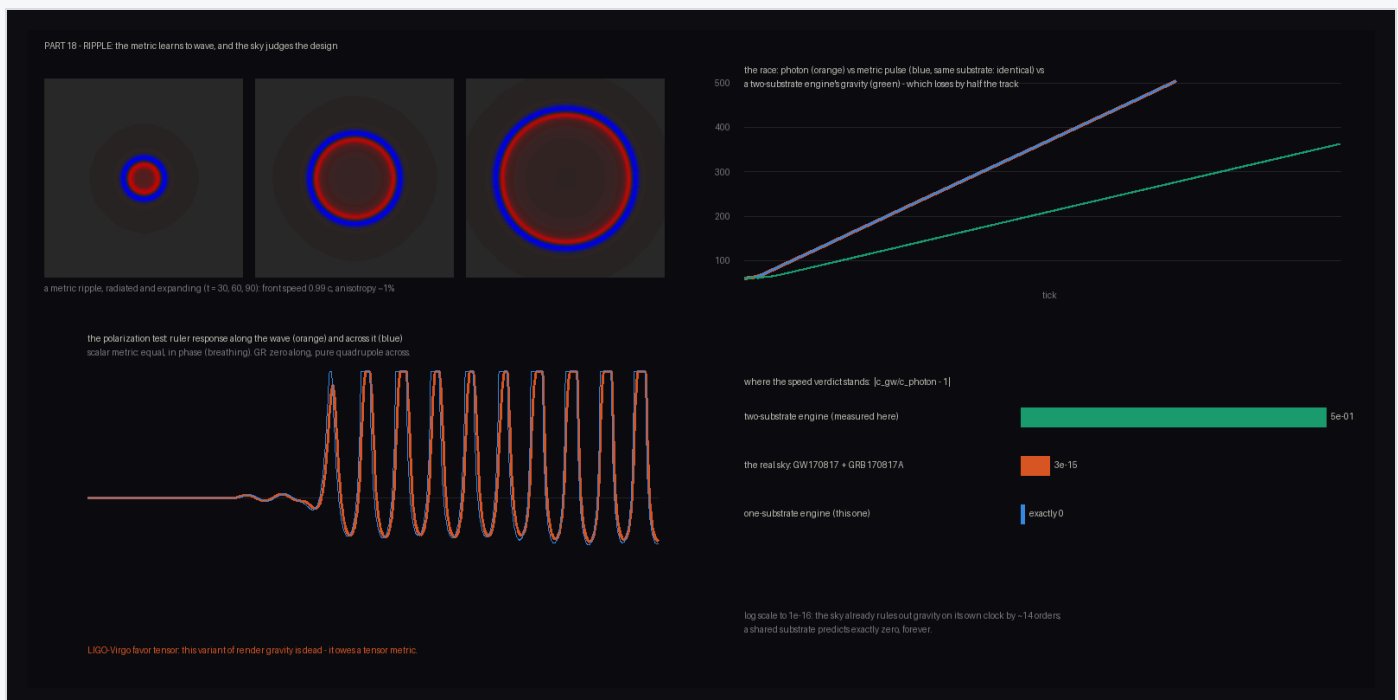
Figure 6. Gravitational-wave comparisons with observation. Top left: a radiated metric ripple (isotropic, front speed 0.99 c ). Top right: the race — photon and metric pulse overlapping exactly; the two-substrate engine's gravity losing by half the track. Bottom left: the breathing-mode strain (equal longitudinal and transverse response) that LIGO–Virgo excludes. Bottom right: the |\Delta c/c| ladder.
