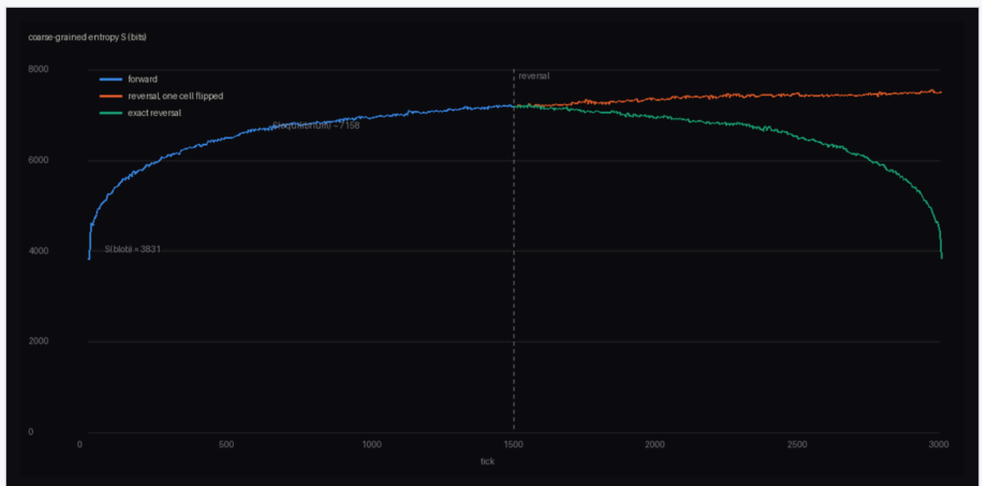
Figure 10. The arrow is not in the laws. Entropy rises (blue), retraces exactly under reversal (green), and clings to equilibrium when one cell was flipped first (orange).
