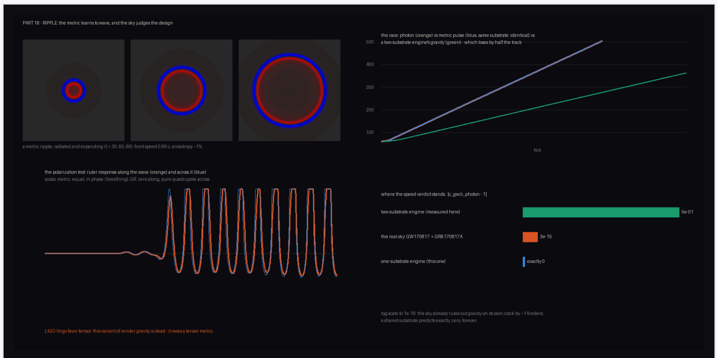
Figure 5. The races the sky already ran. Top left: a radiated metric ripple (isotropic, front speed 0.99c). Top right: the race — photon and metric pulse overlapping exactly; the two-substrate engine's gravity losing by half the track. Bottom left: the breathing-mode strain (equal longitudinal and transverse response) that LIGO–Virgo excludes. Bottom right: the |\Delta c/c| ladder.
