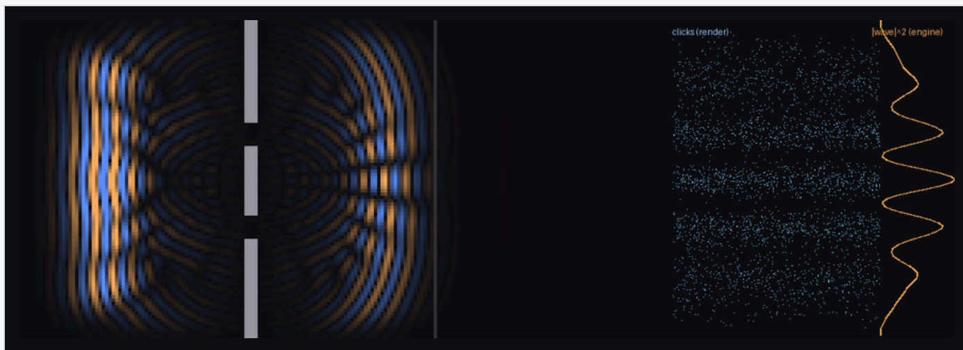
Figure 8. Duality as architecture. Left: the engine's wave interferes through both slits. Right: the renderer's discrete clicks reproduce |\text{wave}|^2 statistically.
