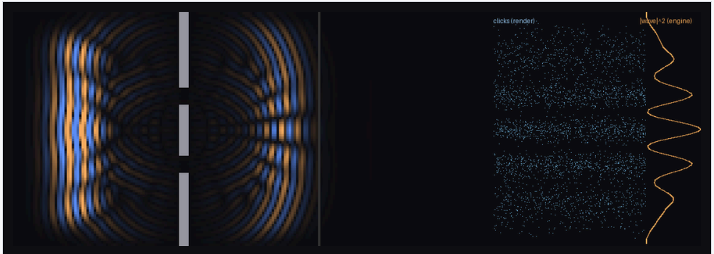
Figure 6. Duality as architecture. Left: the engine's wave interferes through both slits. Right: the renderer's discrete clicks reproduce |\text{wave}|^2 statistically.
