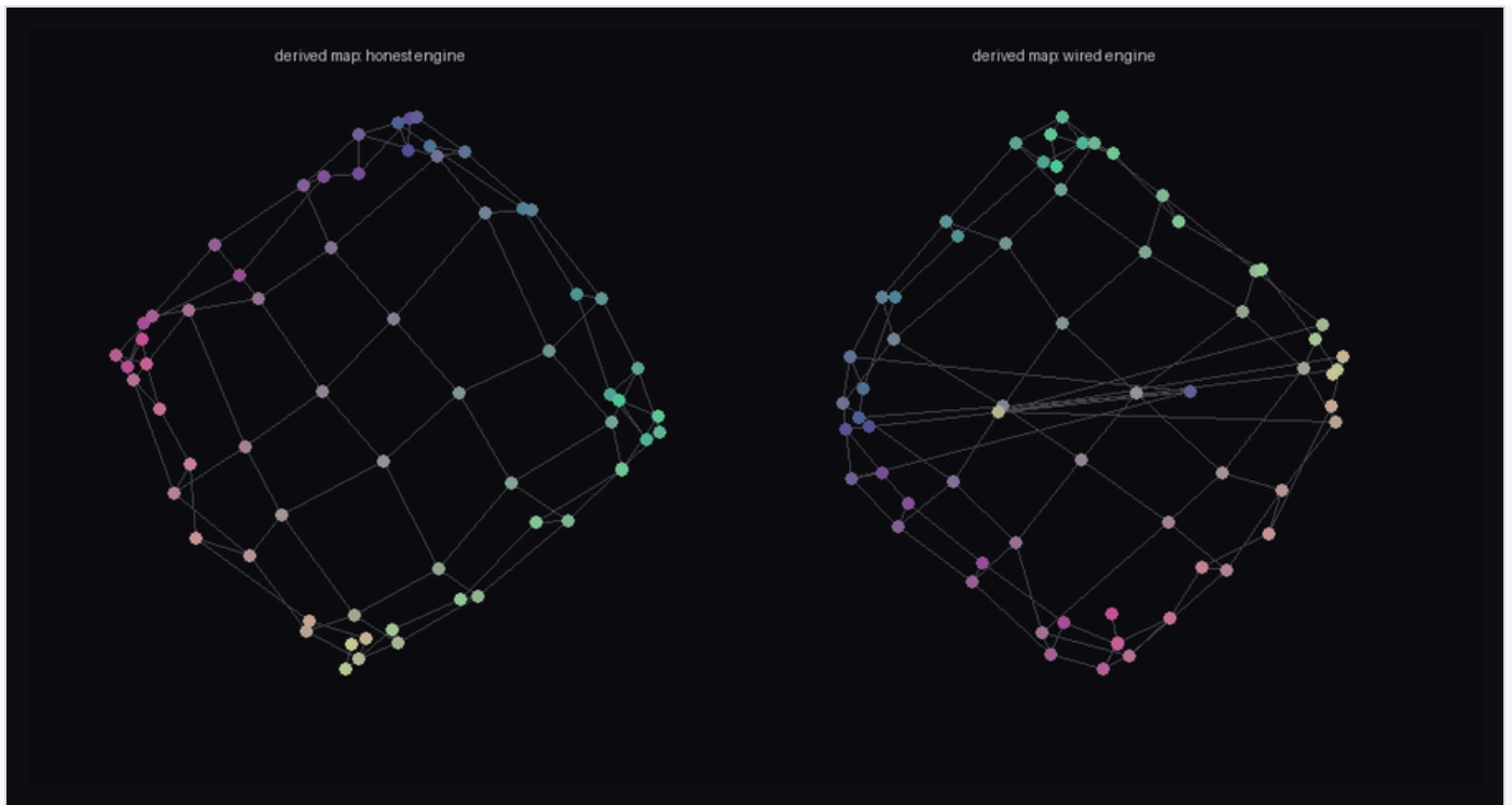
Figure 2. Geometry derived purely from causal structure (no cell index used as a position). Left: honest engine \rightarrow flat mesh. Right: engine with a wired shortcut \rightarrow the derived metric grows a wormhole.
