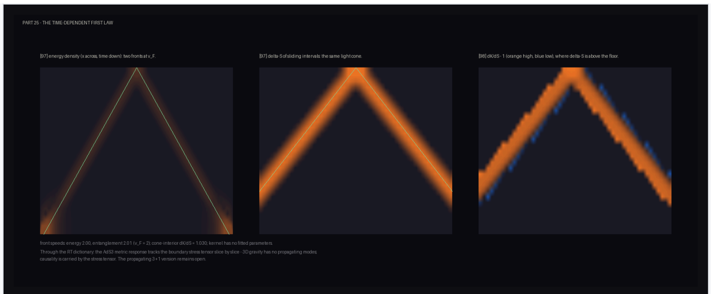
Figure 9. The time-dependent first law. Left: energy density of the released warm region (position across, time down) — two fronts at the Fermi velocity. Center: the entanglement of sliding intervals shows the same light cone. Right: the ratio of the kernel prediction to the measured \delta S , within a few percent of one wherever the signal is above the measurement floor.
