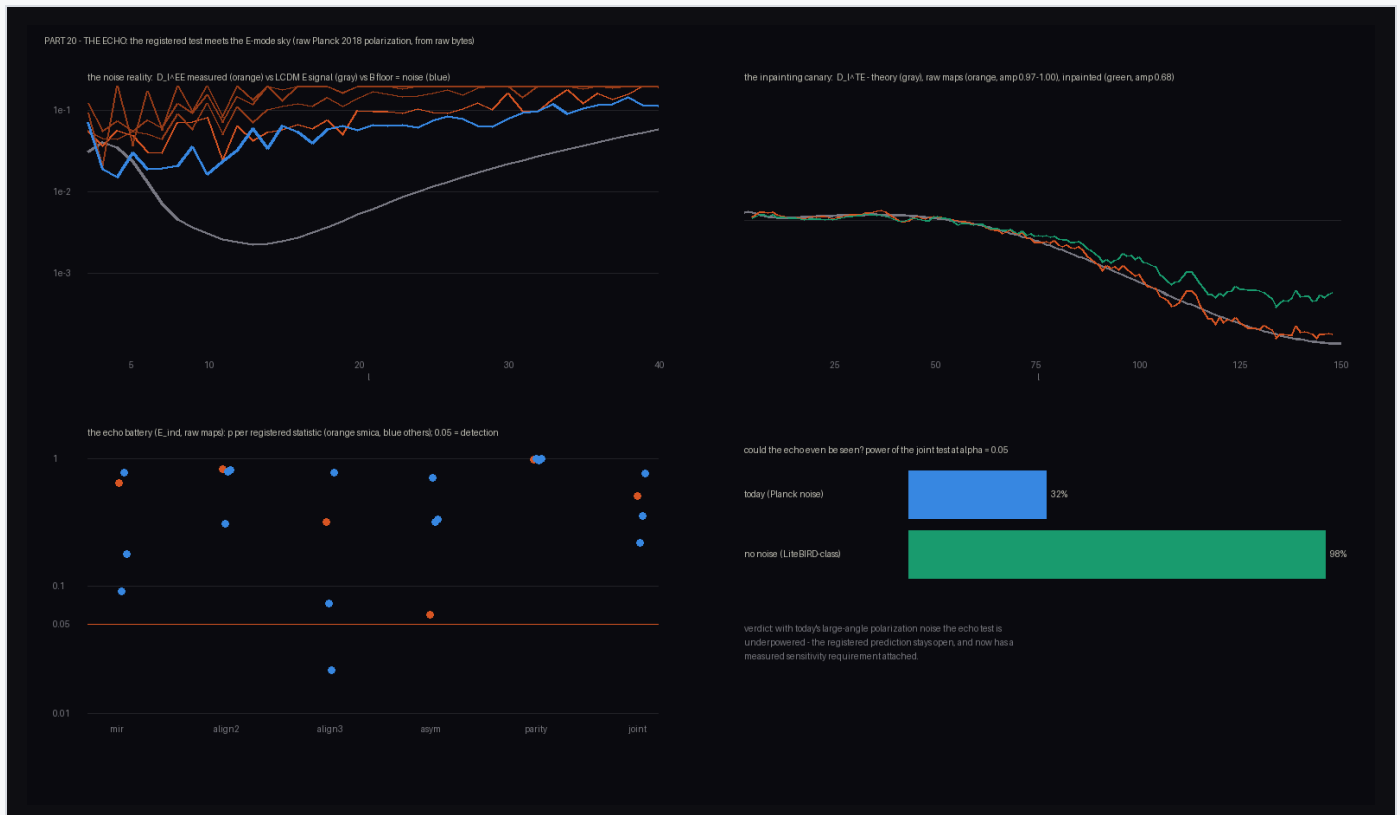
Figure 25. The echo test. Top left: the noise reality — measured EE (orange) sits on the B-mode floor (blue) rather than the \Lambda CDM E signal (gray) beyond \ell \approx 8 . Top right: the inpainting canary in TE. Bottom: the registered-axis battery (no
