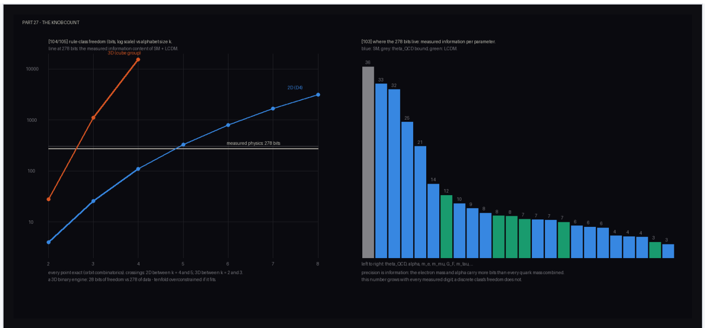
Figure 1. The knob count. Left: exact rule-class freedom in bits against alphabet size for the 2D and 3D constraint ledgers, crossing the measured 278-bit information content of the Standard Model and \Lambda CDM between k = 4 and 5 (2D) and between k = 2 and 3 (3D). Right: where the 278 bits live — measured information per parameter; precision is information, so the electron mass and the fine-structure constant outweigh every quark mass combined.
