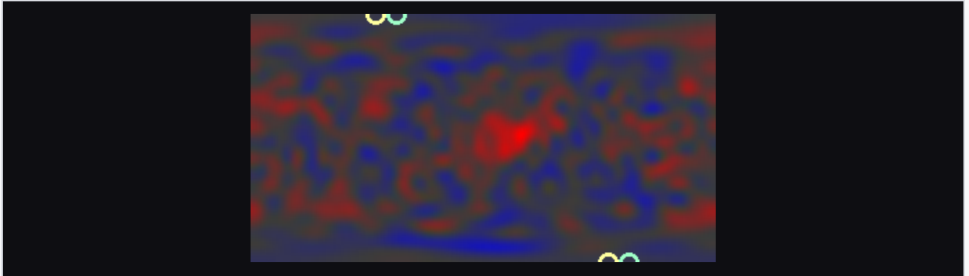
Figure 23. A synthetic sky carrying the three observed anomalies at published amplitudes; rings mark the aligned quadrupole and octupole axes.
