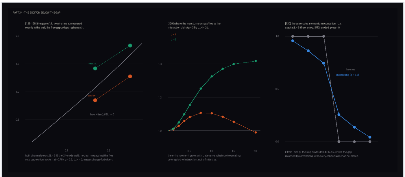
Figure 22. The lowest excitation is charged. Left: the two interacting channels against the free gap collapsing as 4 \tan(\pi/2L) , both measured exactly at L = 4 and 6 . Center: the gap-to-free ratio as a single dial scales the whole interaction. Right: the momentum occupation, whose Fermi step erodes to 0.49 without closing.
