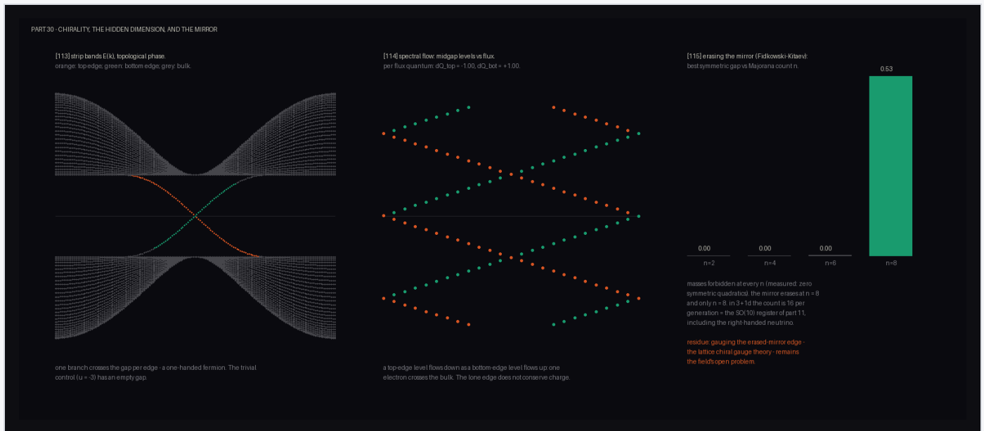
Figure 18. Chirality and the mirror. Left: the Chern strip's bands — one chiral branch crossing the gap per edge, the twin spatially banished. Center: spectral flow under flux — one electron pumped through the bulk per flux quantum, the anomaly as measured bookkeeping. Right: the Fidkowski–Kitaev measurement — symmetric interactions erase the Majorana mirror multiplet at count eight and only count eight.
