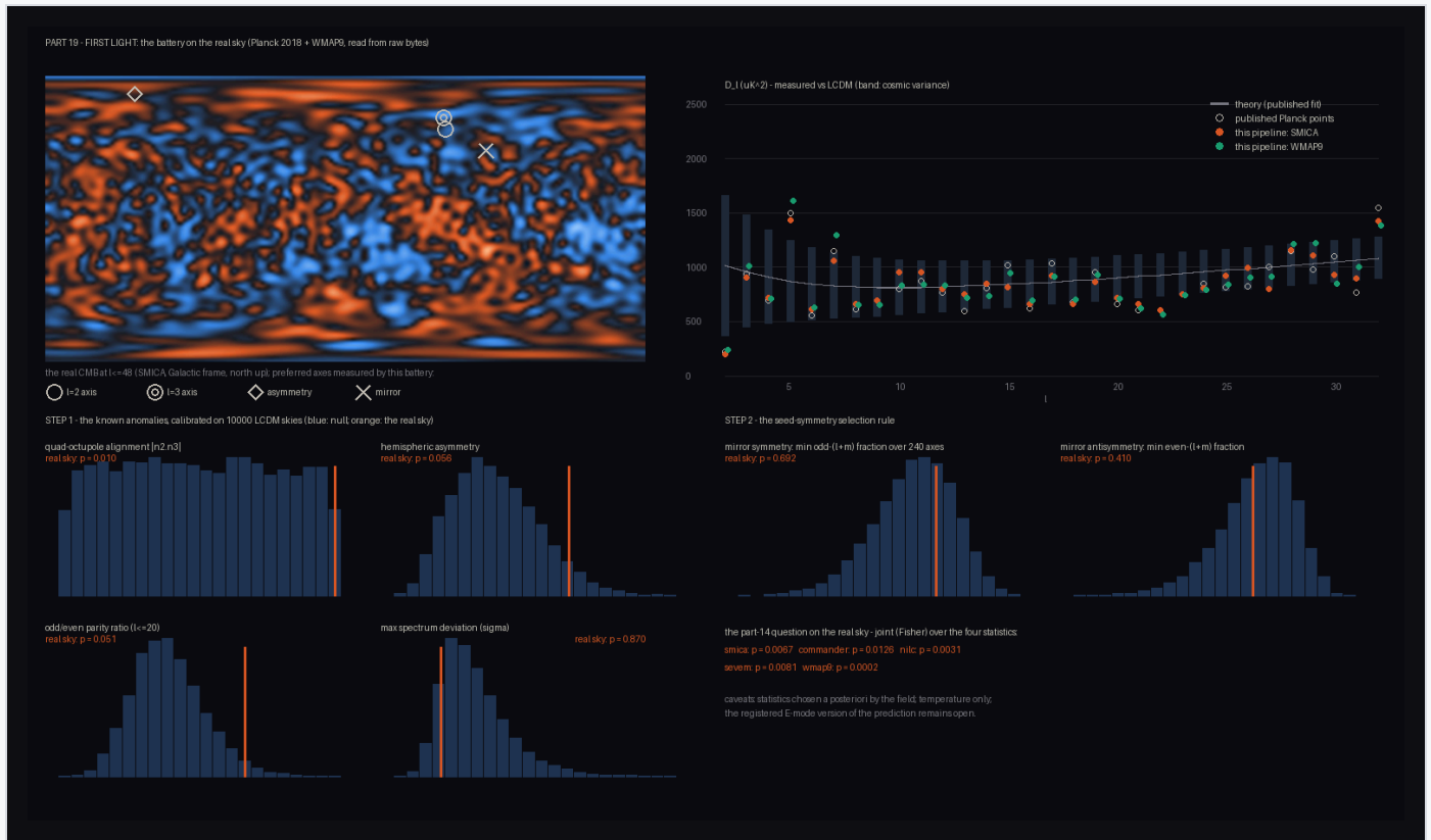
Figure 22. First light: the battery on the real sky. Left: the measured CMB (SMICA, \ell \leq 48 ) with the battery's preferred axes — the two rings nearly touching are the aligned quadrupole and octupole. Right: the from-raw-bytes spectrum against \Lambda CDM (the low quadrupole at far left). Below: each statistic against its 10,000-sky null (orange: the real sky).
