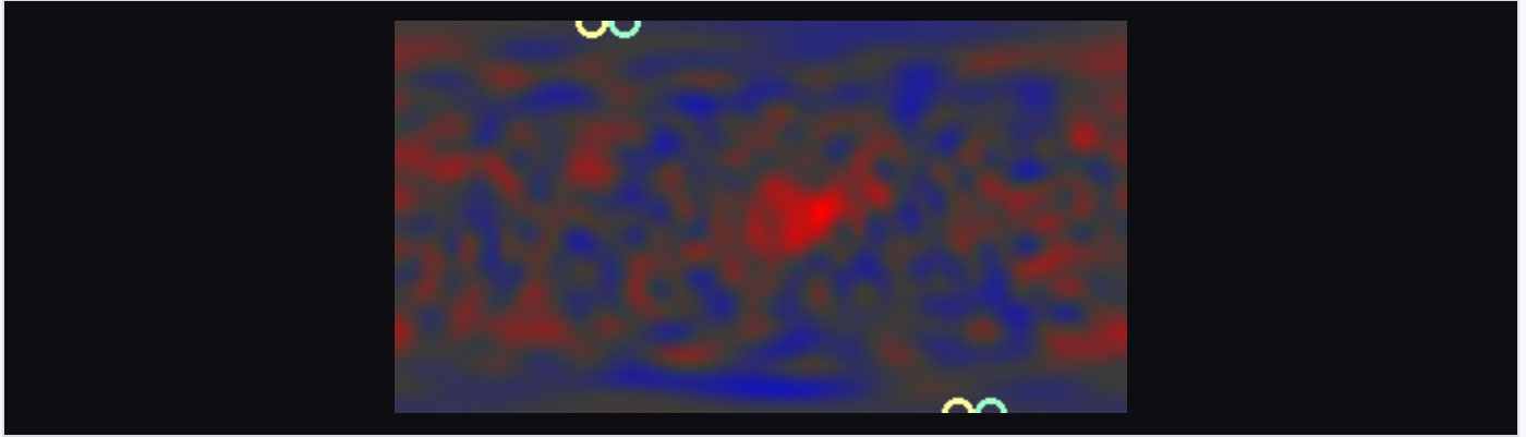
Figure 21. A synthetic sky carrying the three observed anomalies at published amplitudes; rings mark the aligned quadrupole and octupole axes.
