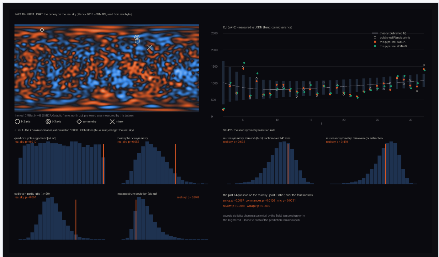
Figure 23. First light: the battery on the real sky. Left: the measured CMB (SMICA, \ell \leq 48 ) with the battery's preferred axes — the two rings nearly touching are the aligned quadrupole and octupole. Right: the from-raw-bytes spectrum against \Lambda CDM (the low quadrupole at far left). Below: each statistic against its 10,000-sky null (orange: the real sky).
