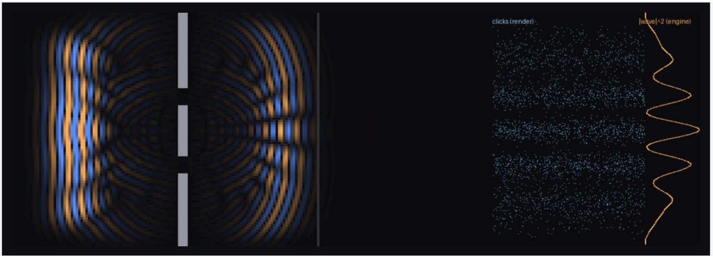
Figure 5. Duality as architecture. Left: the engine's wave interferes through both slits. Right: the renderer's discrete clicks reproduce |\text{wave}|^2 statistically.
