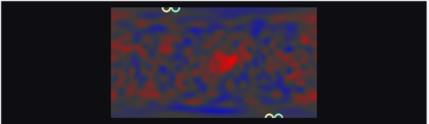
Figure 19. A synthetic sky carrying the three observed anomalies at published amplitudes; rings mark the aligned quadrupole and octupole axes.
