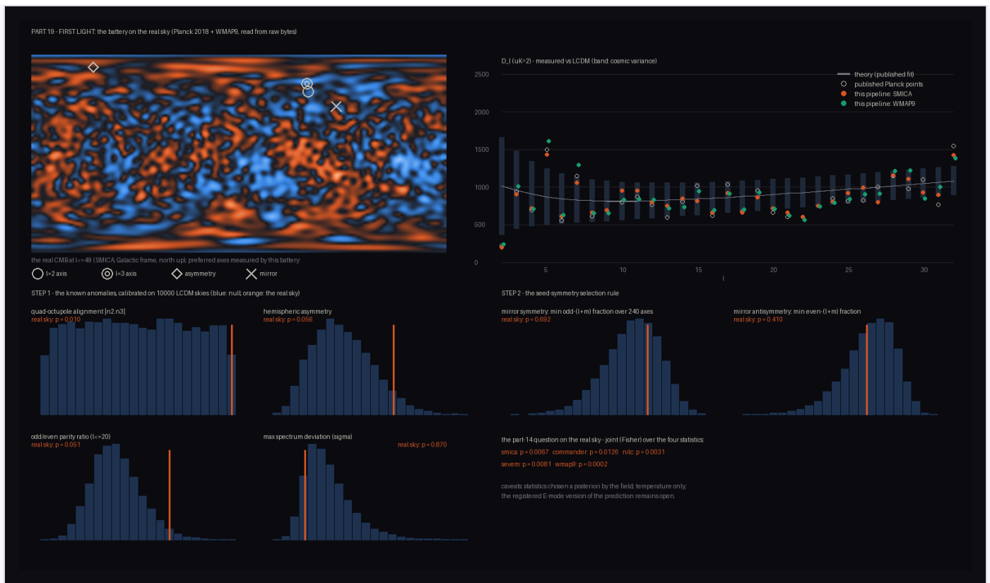
Figure 21. First light: the battery on the real sky. Left: the measured CMB (SMICA, \ell \leq 48 ) with the battery's preferred axes — the two rings nearly touching are the aligned quadrupole and octupole. Right: the from-raw-bytes spectrum against \Lambda CDM (the low quadrupole at far left). Below: each statistic against its 10,000-sky null (orange: the real sky).
