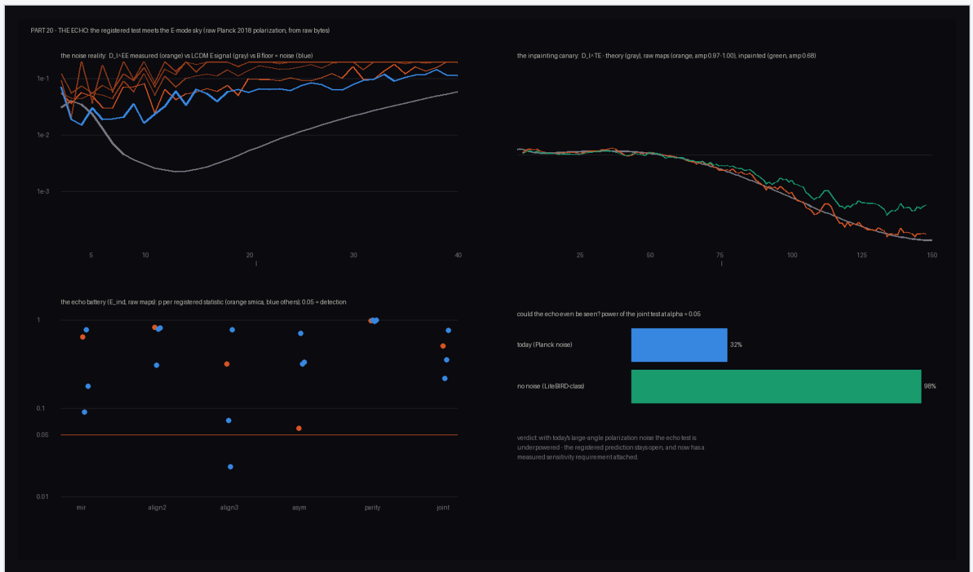
Figure 22. The echo test. Top left: the noise reality — measured EE (orange) sits on the B-mode floor (blue) rather than the \Lambda CDM E signal (gray) beyond \ell \approx 8 . Top right: the inpainting canary in TE. Bottom: the registered-axis battery (no echo) and the measured power of the test — 32% at today's noise, 98% at LiteBIRD-class.
