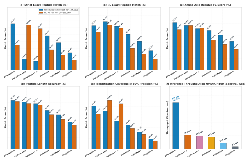
Comprehensive De Novo Peptide Sequencing Benchmark Across Full Test Splits ( N = 369,532 Spectra)
