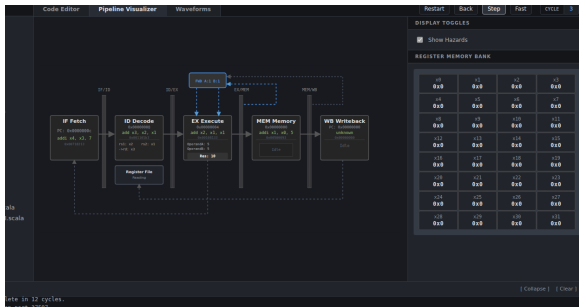
(a) Level 2 forwarding, cycle 3.
