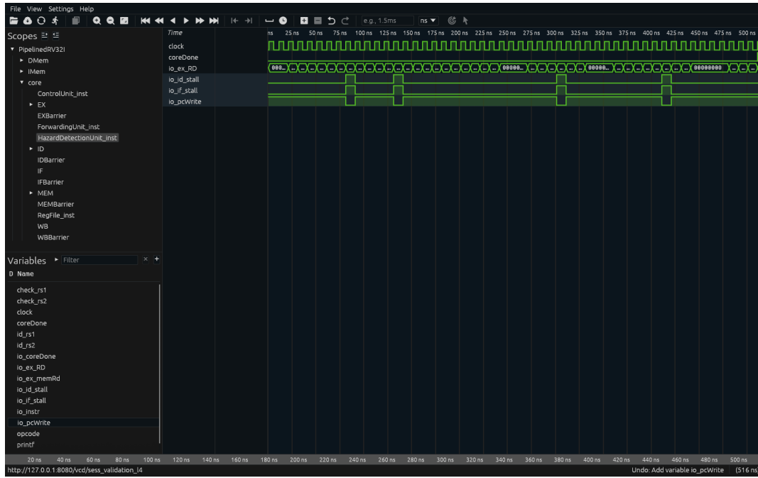
Figure 5: Generated Level 4 waveform displayed in the bundled Surfer viewer. The selected clock and processor debug signals complement the cycle-level pipeline representation.
