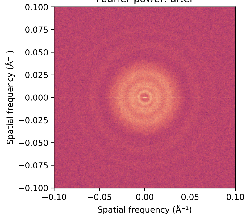
Fourier power: after
