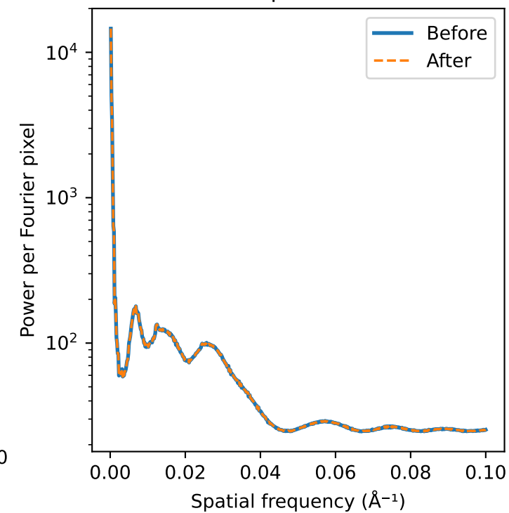
Mean radial power: all 61 tilts
