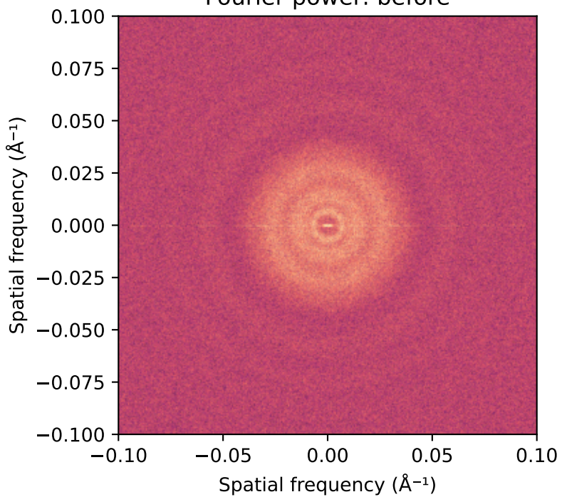
Fourier power: before
