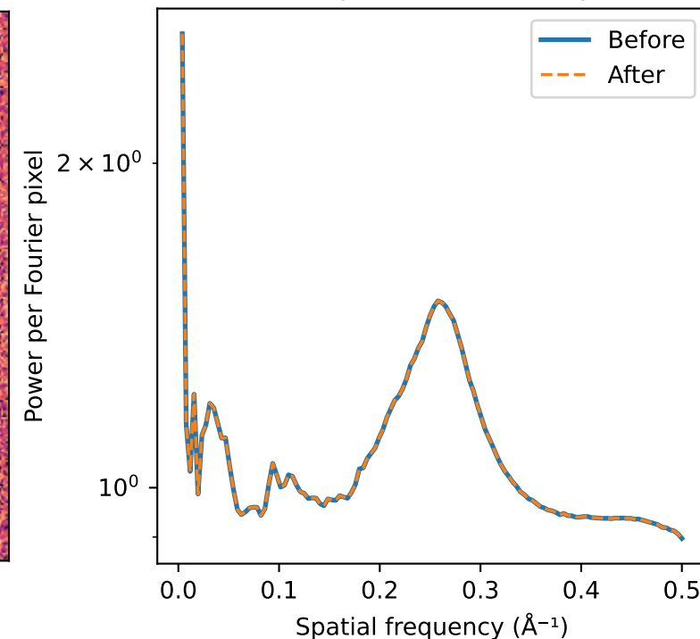
Mean radial power: all 3,000 particles
