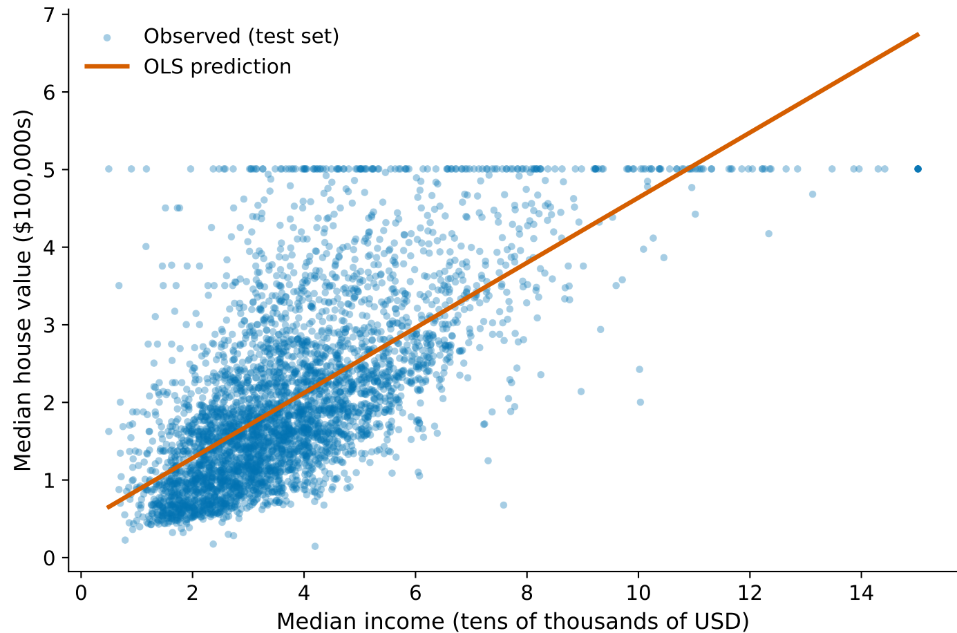
Test observations and the fitted OLS line
