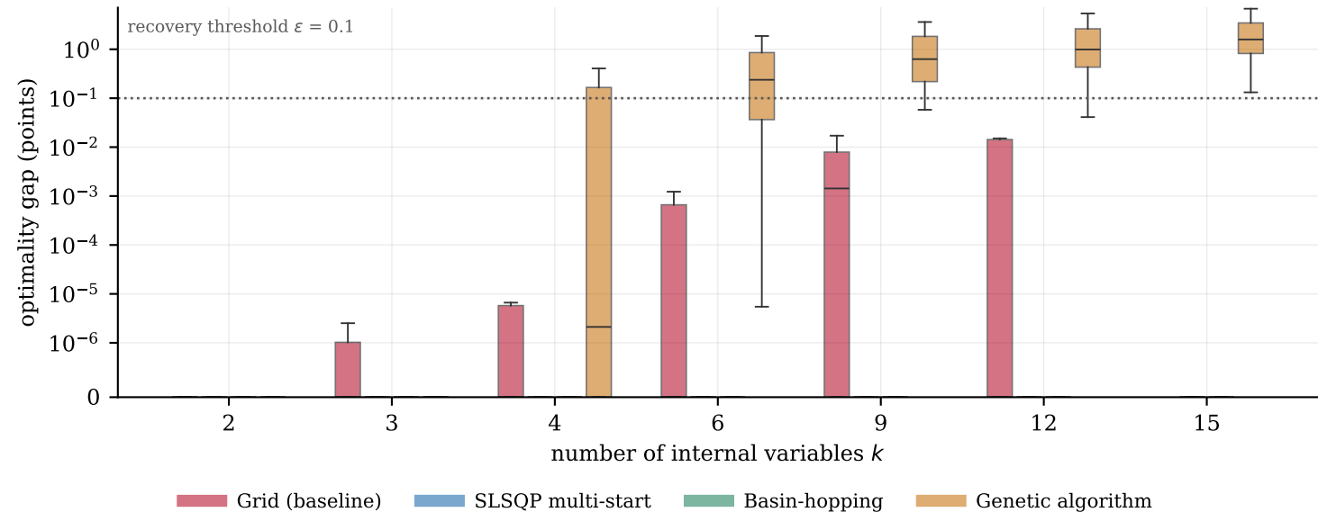
Optimality gap by method (negative gaps clipped to zero for display)
