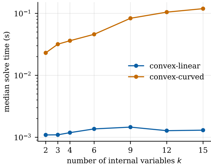
SCIP solve cost
