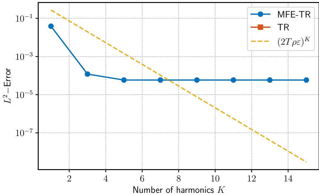
K convergence
