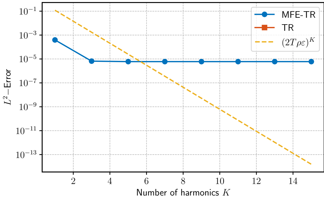
K convergence
