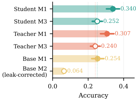
(a) All accuracy metrics 95% clustered bootstrap CI
