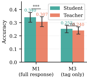
(b) M1 vs M3: CoT signature S>T on M1; parity on M3
