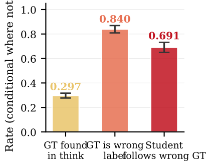
(c) GT contamination cascade SFT format-slot artifact
