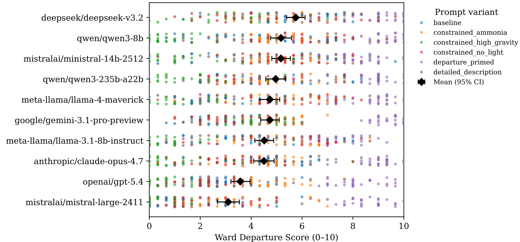
Ward Departure Score: per-model distribution (points) and mean (95% bootstrap CI)
