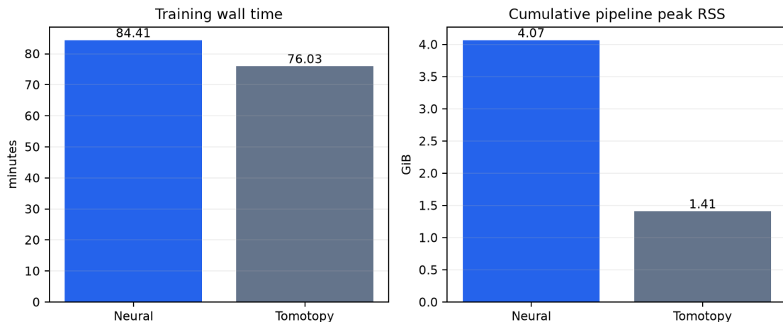
Figure 4: Six-worker training time and cumulative pipeline peak RSS from the fresh neural and hash-verified Tomotopy source processes. RSS is not isolated to either training stage.
