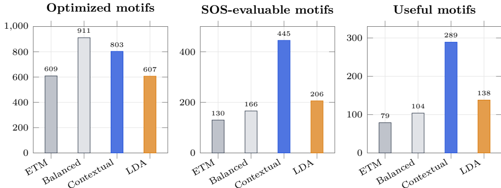
Figure 3: Validation motif inventory after successive chemical filters. ETM is the canonical Embedded Topic Model with fixed train-only spectral-word coordinates and dense softmax document mixtures. Balanced is the same ETM with separate 50/50 fragment and neutral-loss decoder normalization. Contextual is the complete Contextual Sparse ETM, which adds contextual top-2 posterior evidence and 1.5-entmax to Balanced. LDA is Tomotopy 0.13.0 latent Dirichlet allocation. Optimized means that Mass2Motif Annotation Guidance (MAG) retains at least one fragment or loss; SOS-evaluable means that the substructure overlap score can be computed from at least one associated molecule; useful means SOS at least 0.6. All four models use K = 1000 and the same frozen training/validation split and chemical-evaluation protocol.
