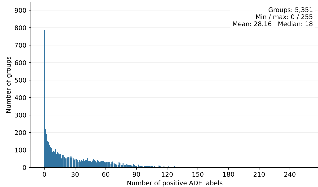
PT: positive ADEs per group
