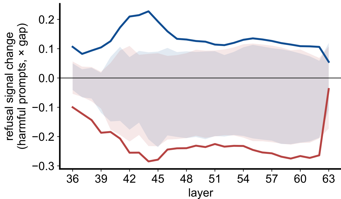
Qwen2.5-32B
