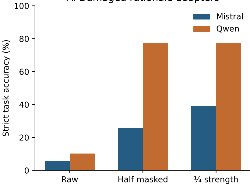
A. Damaged rationale adapters
